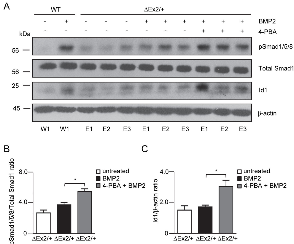
Figure 6. Treatment with 4-PBA rescues signaling defects in Bmpr2 \Delta Ex2/+ pulmonary endothelial cells. Individual primary PECs isolates obtained from 1 wild type control and 3 Bmpr2 \Delta Ex2/+ mice were treated with 1mM 4-PBA for 48 hours followed by BMP2 treatment for 4 hours, as indicated. A, Western blot for phospho-Smad1/5/8 and Id1 shows 4-PBA restores phospho-Smad1/5/8 and Id1 expression in Bmpr2 \Delta Ex2/+ PECs to expression levels similar to BMP-stimulated WT PECs. B, Densitometry for phospho-Smad1/5/8 and C, Id1 expressed as ratio to total Smad1 and \beta -actin respectively. Results expressed as mean \pm SEM of three individual PEC isolates per group. One-way ANOVA with post hoc Bonferroni correction, p < 0.05 * \Delta Ex2/+ +BMP2 vs. \Delta Ex2/+ +BMP2+4-PBA.
