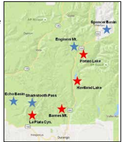
Figure 3. Sampling locations for genetic analysis of. Alpine V. "bellidifolia" represented by blue stars, Montane V. adunca by red stars.
