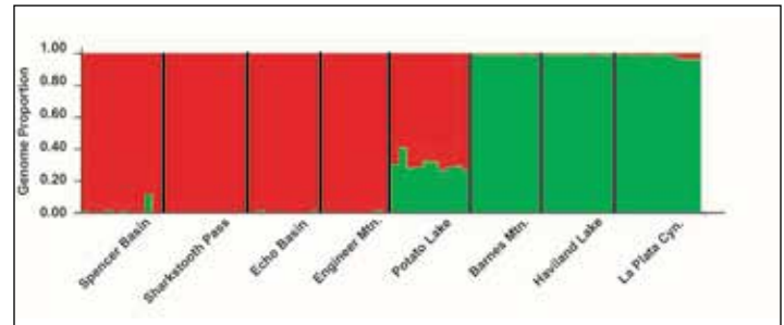
Figure 4. Identification of genetic clusters among populations of Viola adunca from the western San Juan Mountains. See Figure 3 for locations and taxon affinity of populations.
