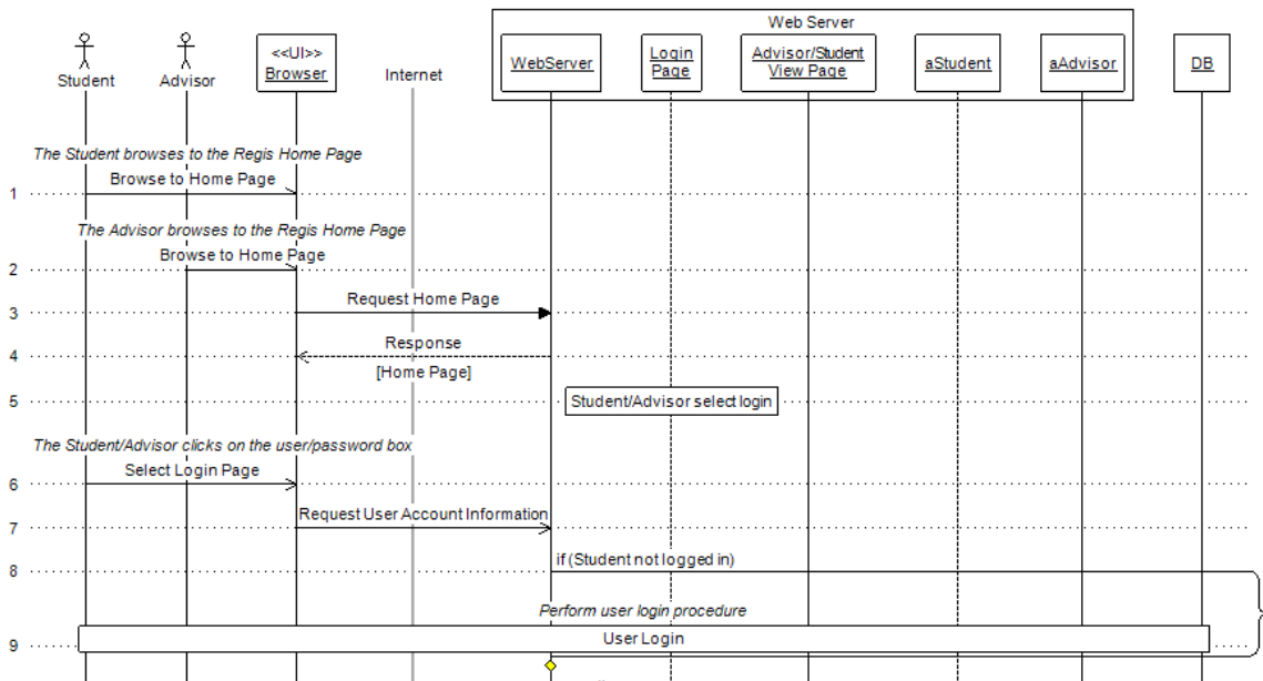
Figure 14. Sequence Diagram part – 1
