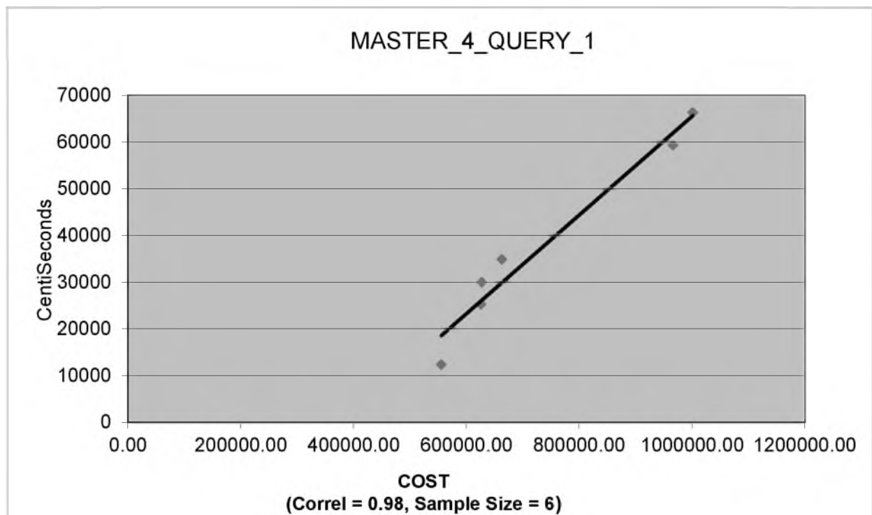
Figure 5.10 – Master_4_Query_1
