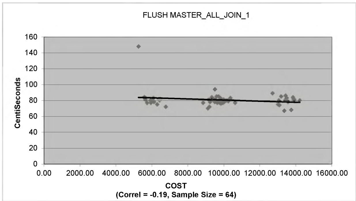
Figure 5.7 – FLUSHED Master_All_Join_1
