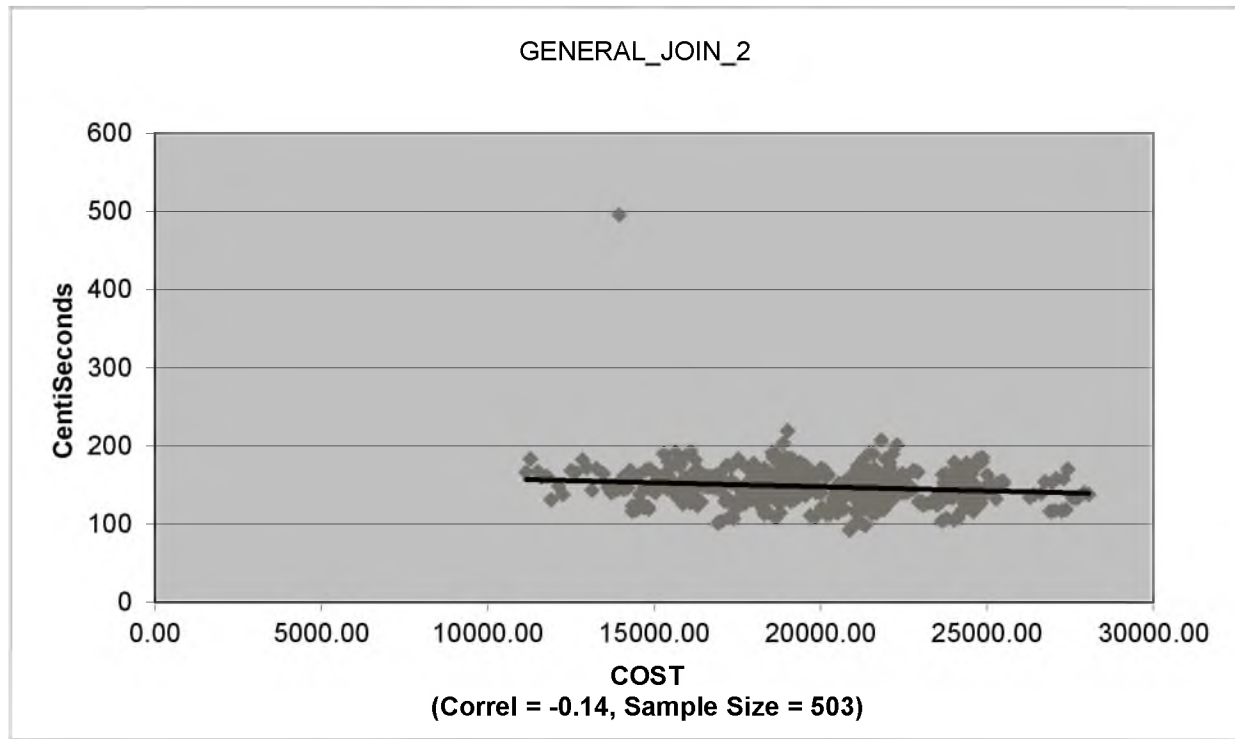
Figure 5.2 – NOT FLUSHED General_Join_2
