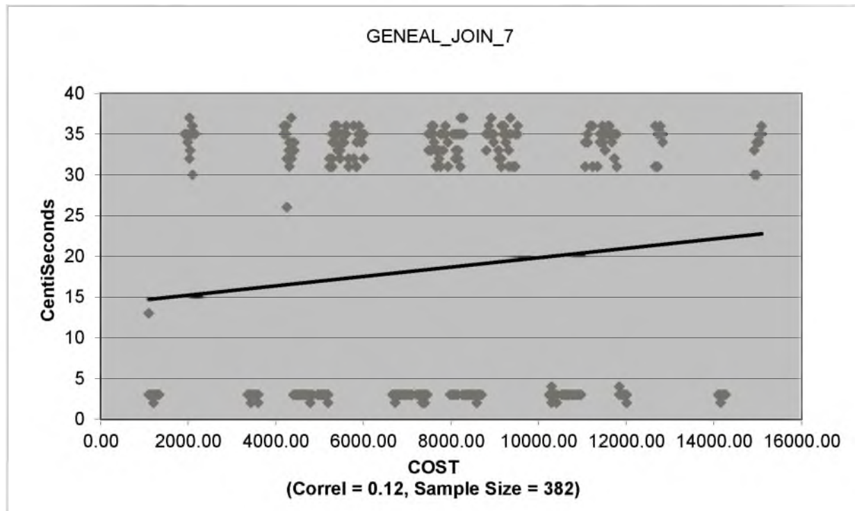
Figure 5.5 – NOT FLUSHED General_Join_7
