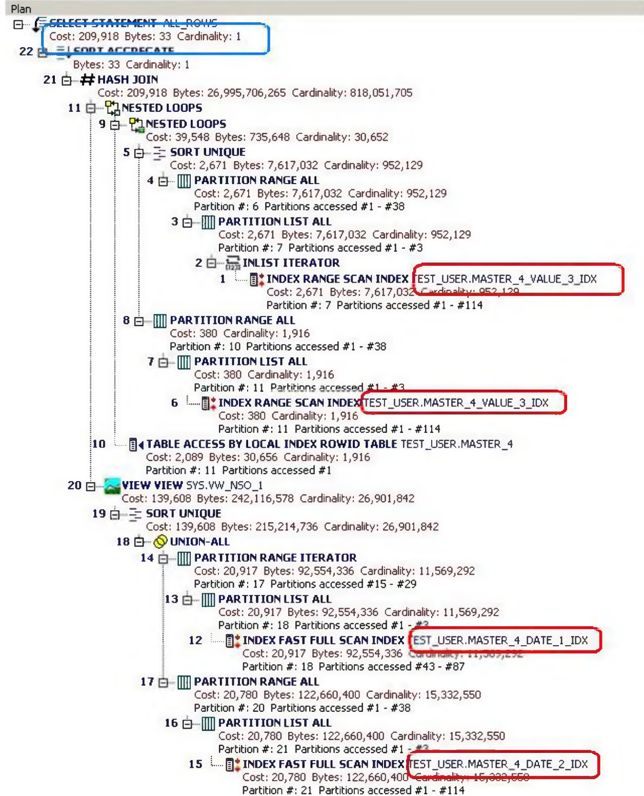
Figure 4.12 – Execution Plan
