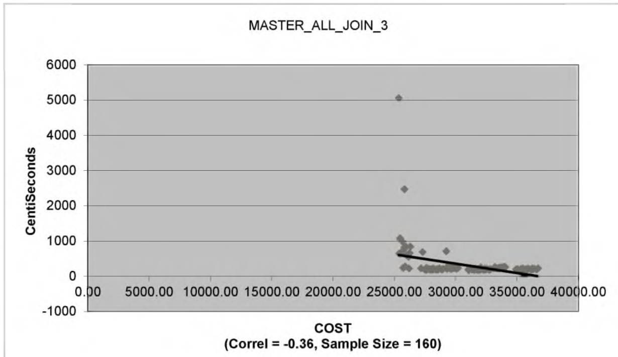
Figure 5.3 – NOT FLUSHED Master_All_Join_3
