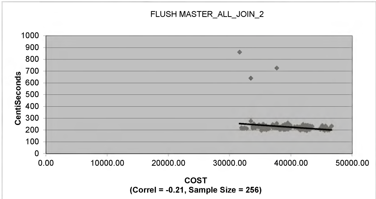
Figure 5.8 – FLUSHED Master_All_Join_2
