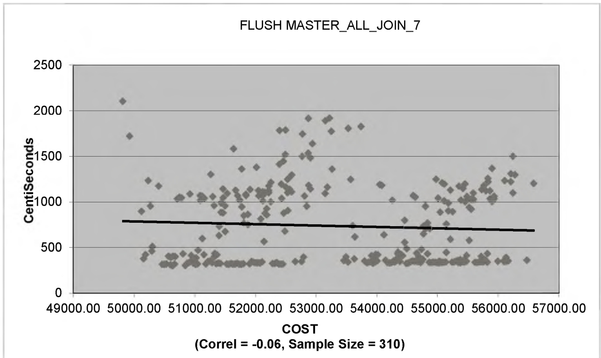
Figure 5.9 – FLUSHED Master_All_Join_7
