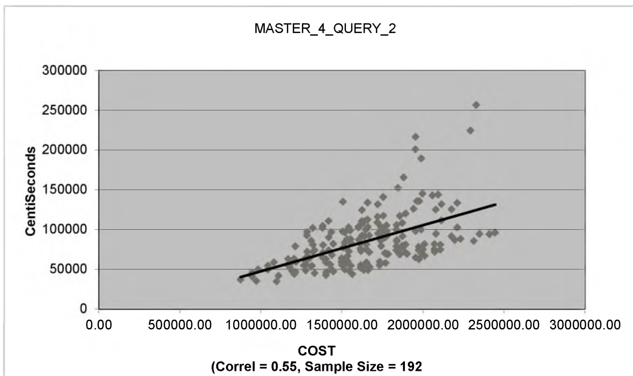
Figure 5.11 – Master_4_Query_2
