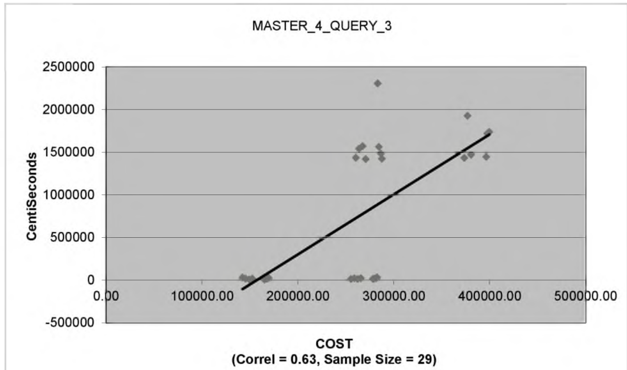
Figure 5.13 – Master_4_Query_3
