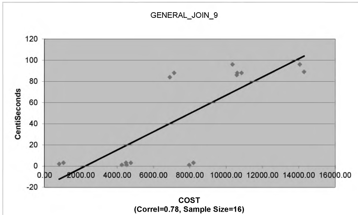
Figure 5.6 – NOT FLUSHED General_Join_9
