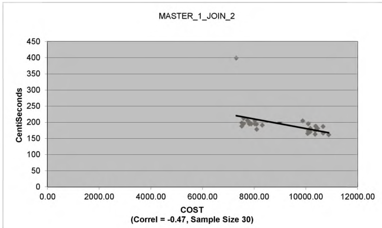
Figure 5.4 – NOT FLUSHED Master_1_Join_2
