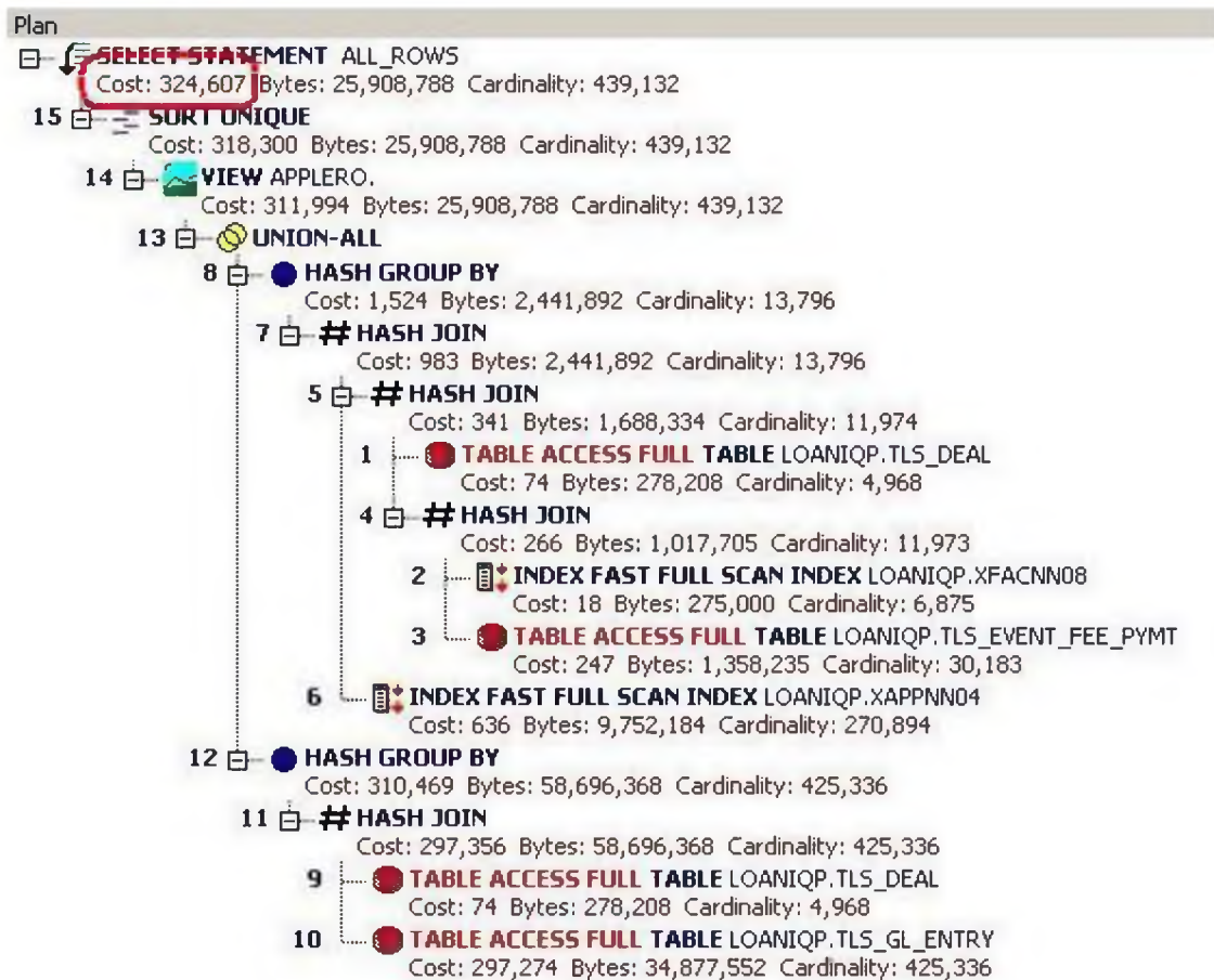
Figure 1.5 -- Using EP for a more complex query
