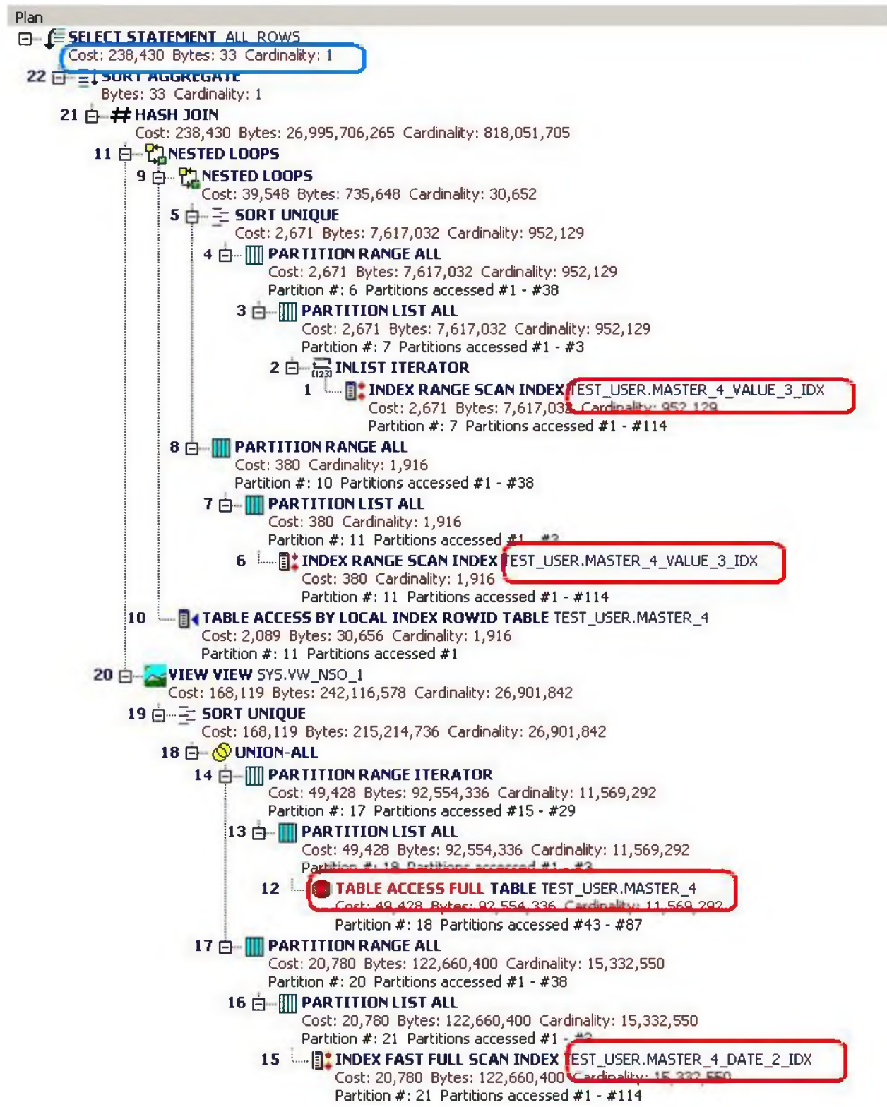
Figure 4.13 - Revised Execution Plan
