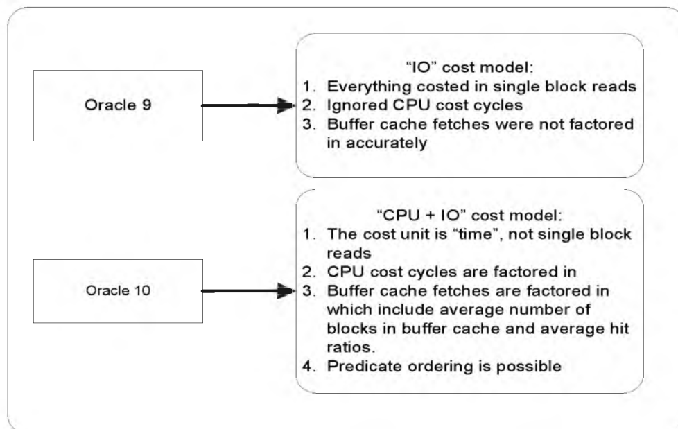
Figure 2.1 -- High level CBO differences
