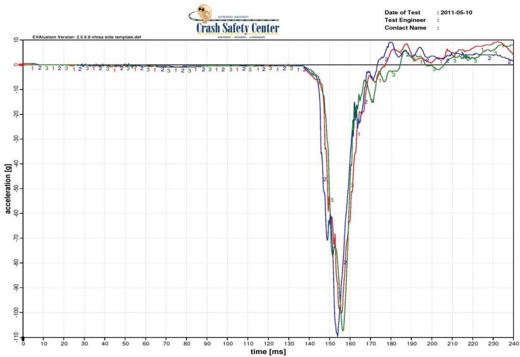
Figure 17: Lateral head and pelvis acceleration plots for SIDE 007 – SIDE 009 using CRABI 12 RF
