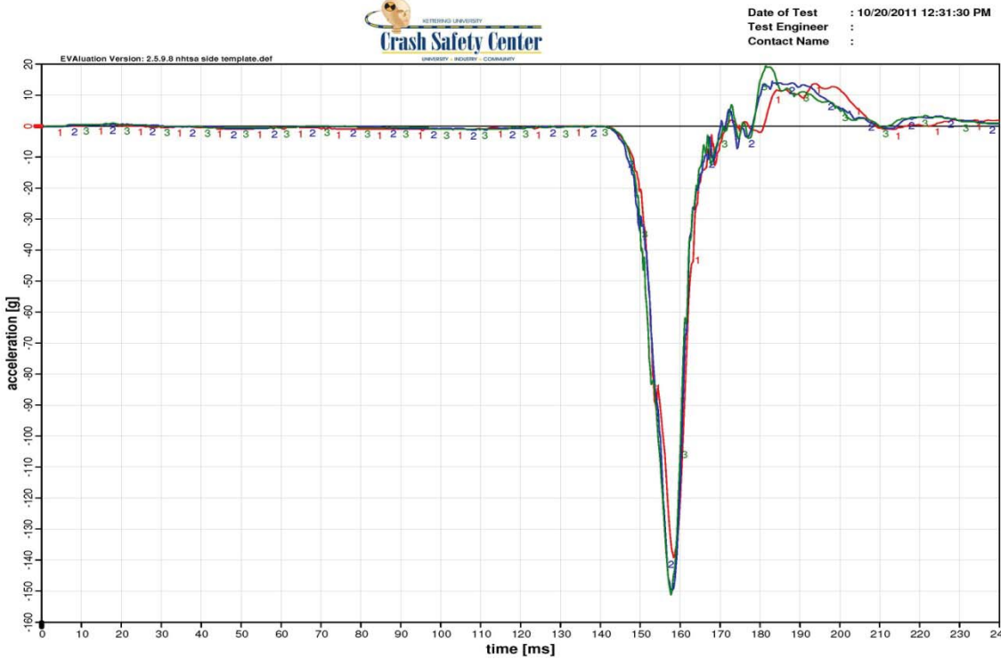
Figure 19: Lateral head and pelvis acceleration plots for SIDE 013 – SIDE 015 using Q3s RF
