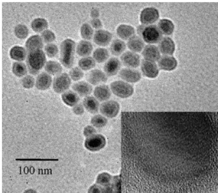
Figure 1. A TEM micrograph of \alpha\text{-MnAs}/\beta\text{-MnAs} core/shell nanoparticles synthesized by the reaction of triphenylarsine oxide and dimanganesedecacarbonyl in the presence of trioctylphosphine oxide. Taken from K Senevirathne, R. Tackett, PR Kharel, G Lawes, K Somaskandan and SL Brock, ACS Nano 3(5), 1129 (2009).
