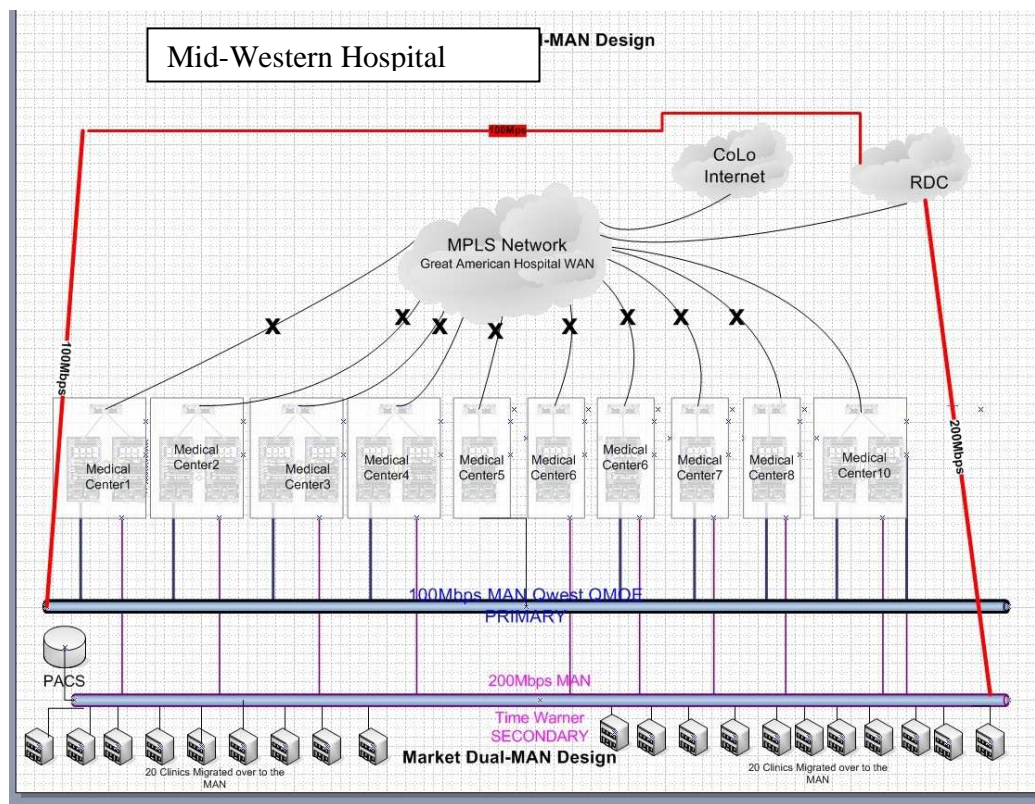
Fig. 4 New Dual-MAN network Diagram (full 24/7 redundant connection)
