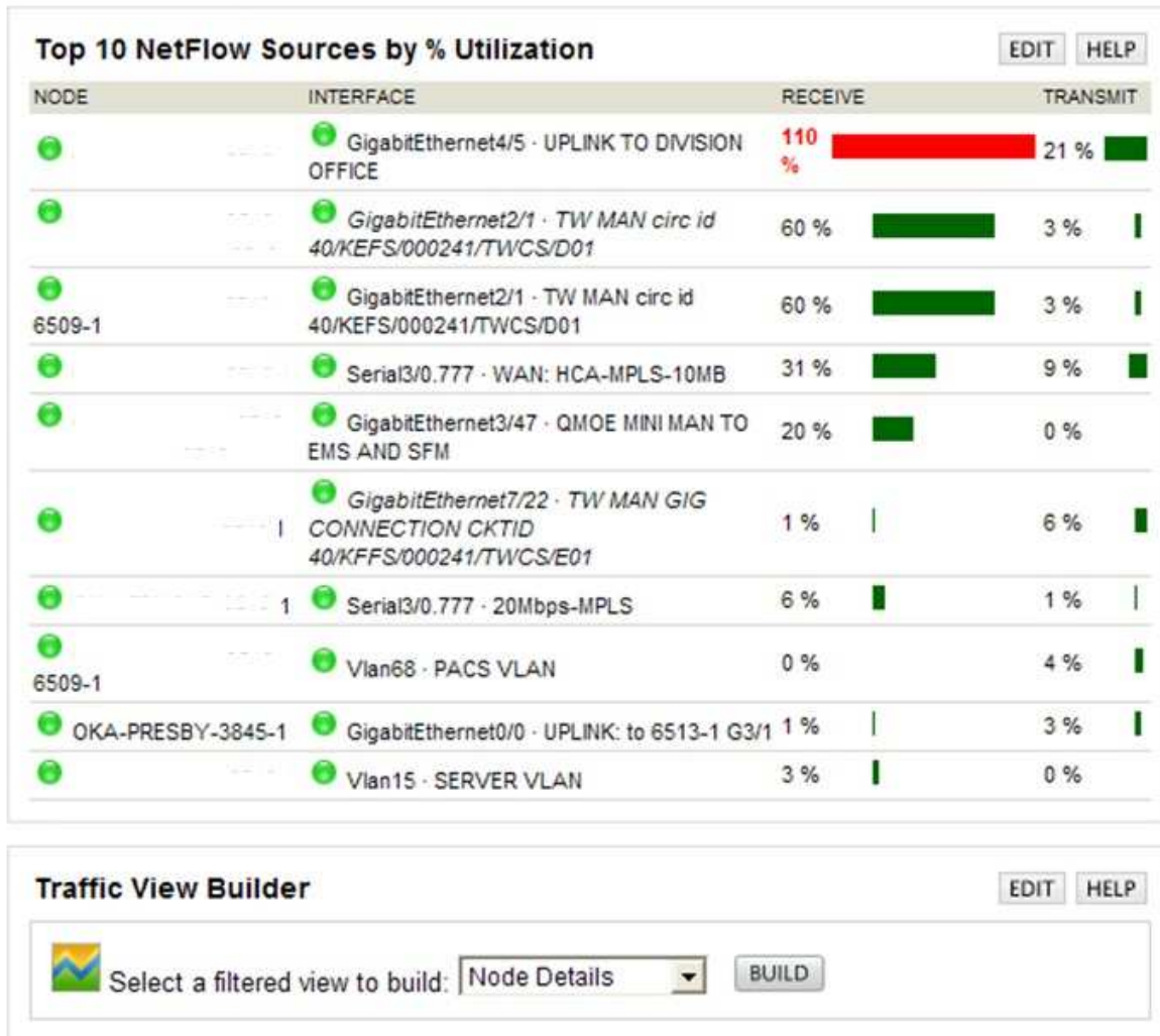
Fig 9A is an example diagram of a sample report from Orion SolarWinds shows percentage of network utilization. The diagram is changed to protect the company’s confidentiality. The data is presented in a clear and organized user interface which allows network monitors to read and interpret data quickly. The Orion SolarWinds tool shows reports of the network interface by percent utilization and volume and memory utilization. This power tool also alerts Network Engineers of Vlan mismatches discovered on the network, status changes and packet information received and transmitted and connection outages or data loss that might affect performance and enterprise functionality.
