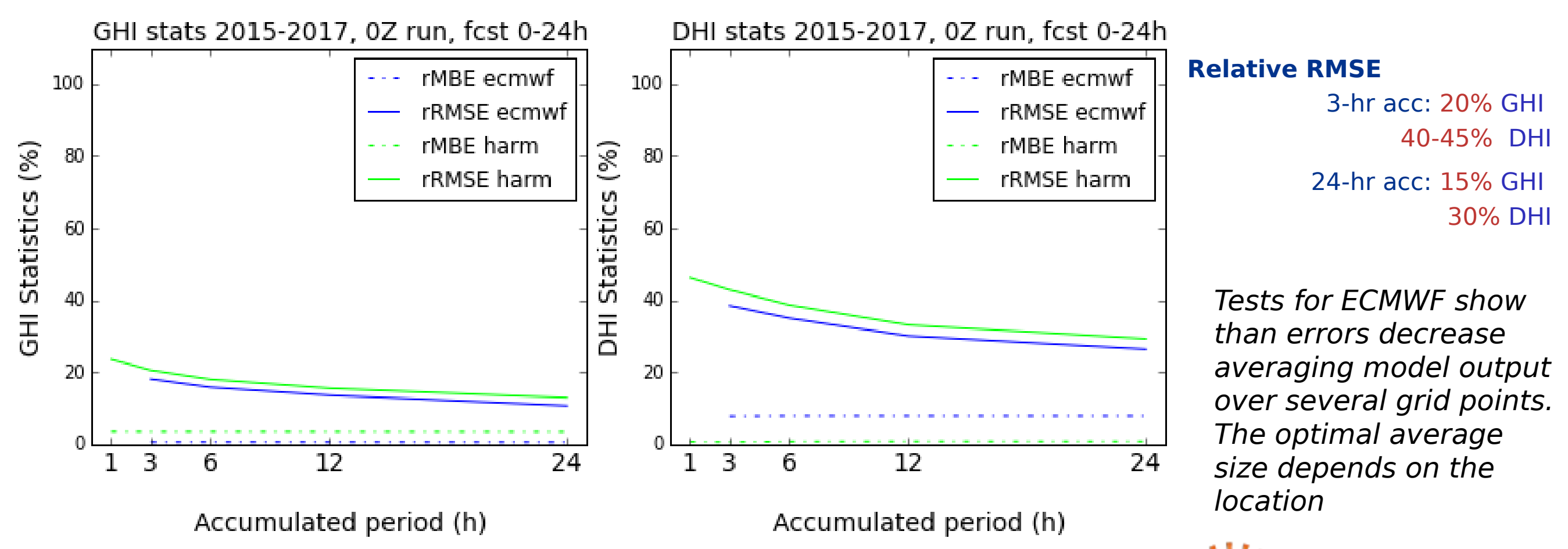
Relative RMSE and BIAS for different accumulations. ECMWF model performs slightly better although HARM-AROME shows lower bias
