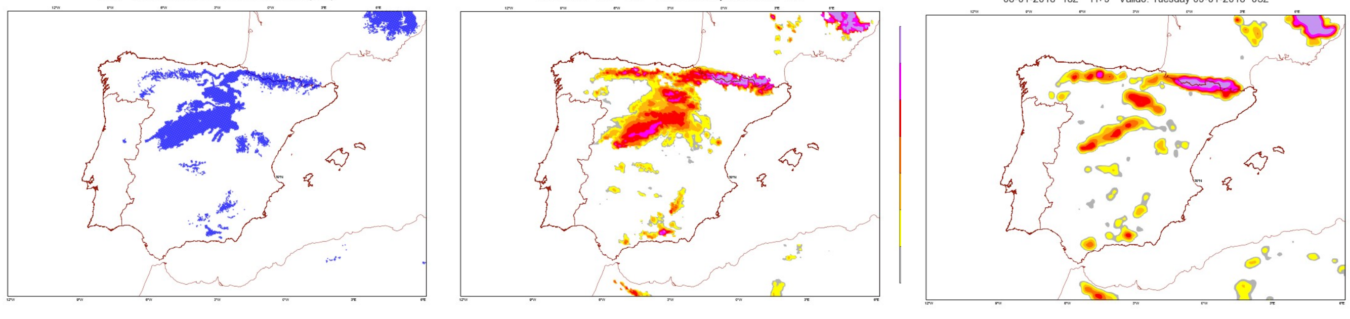
09-01-2018: (a) IMS NOAA/NIC snow cover analysis, (b) HARM-AROME snow depth (c) ECMWF snow depth
