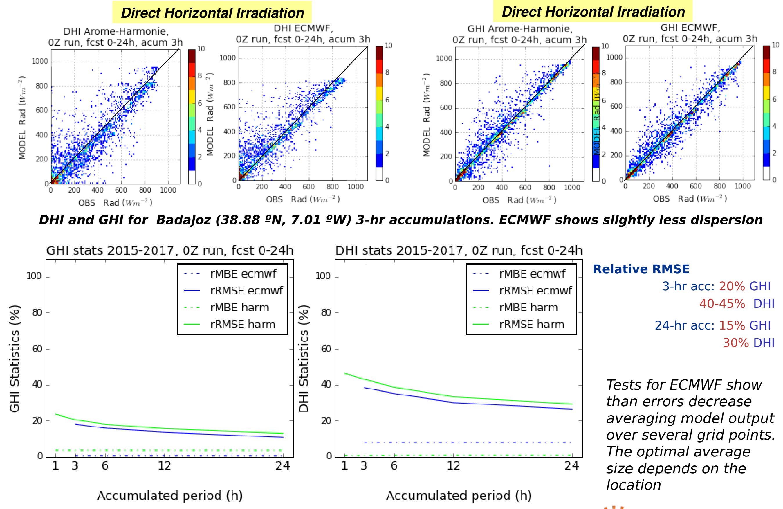
Relative RMSE and BIAS for different accumulations. ECMWF model performs slightly better although HARM-AROME shows lower bias
