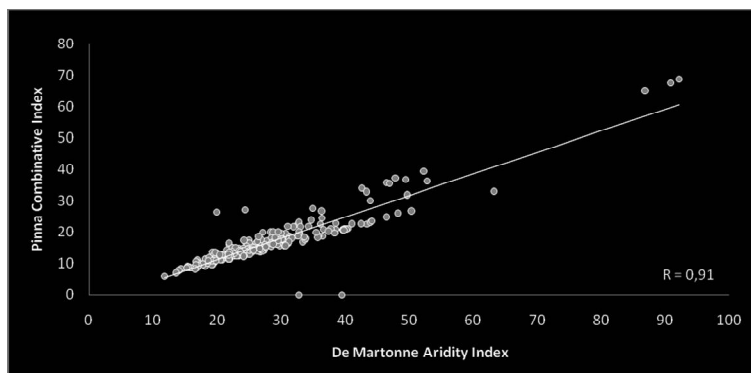
Figure 7: Statistical analysis between the indices of De Martonne and Pinna.
