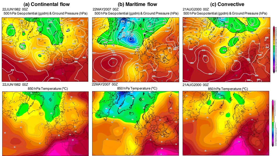
Fig. 2: Examples of the classified synoptic situations: (a) continental flow, (b) maritime flow and (c) convective situation. 500 hPa geopotential and ground pressure (top), and 850 hPa Temperature (bottom) reanalysis data from NCEP (data provided online at www.wetterzentrale.de ). In the top panels T represents a low pressure system.
