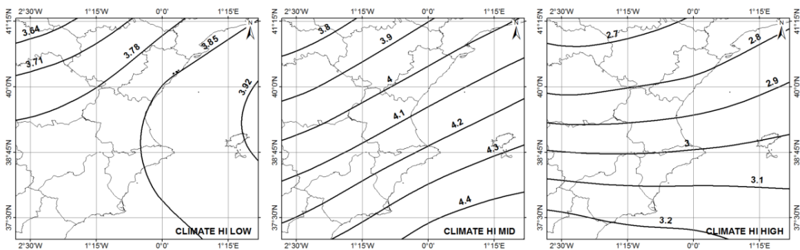
Fig. 3: Spatial distribution of the climatological averages for each variant of the HI calculated for the whole period.
