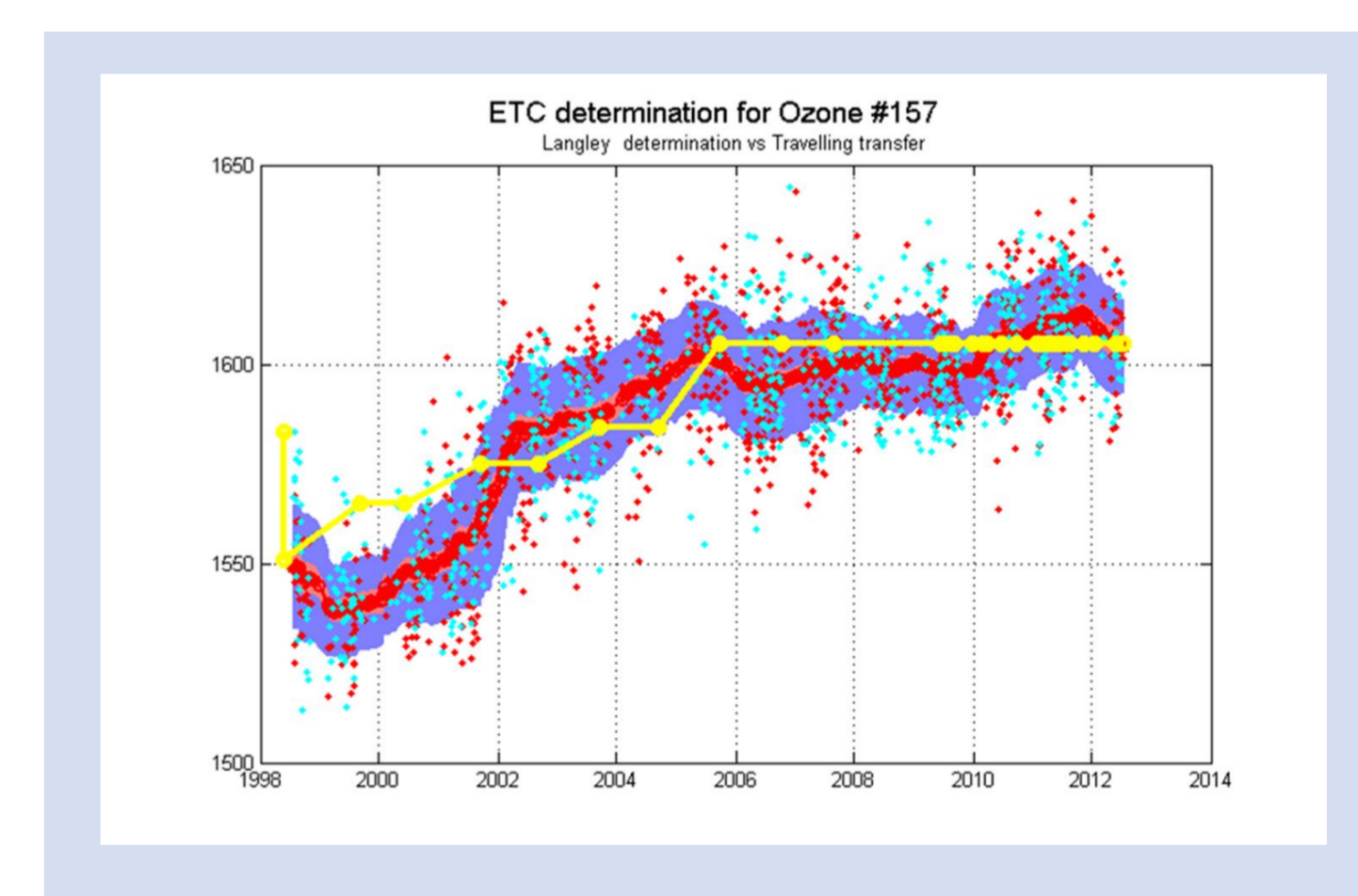
Figure 4: Long term 1998-2012 comparison of Langley calibration (red line) and ETC transferred by the IOS travelling instrument 17
