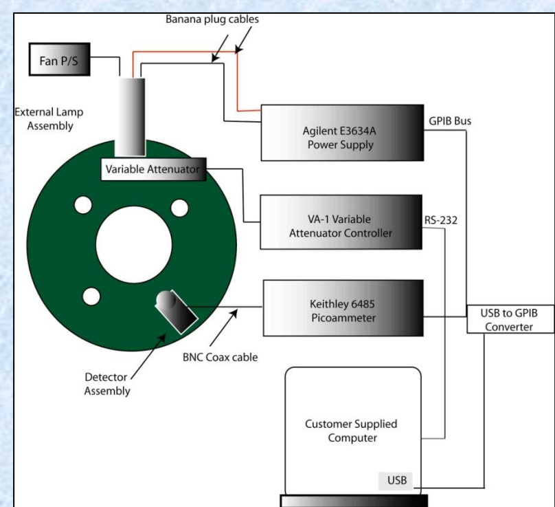
Figure 1. System block diagram and wiring scheme
