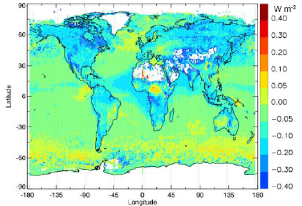
Total AOD deviation (Aerocom mean – MODIS year 2000)
