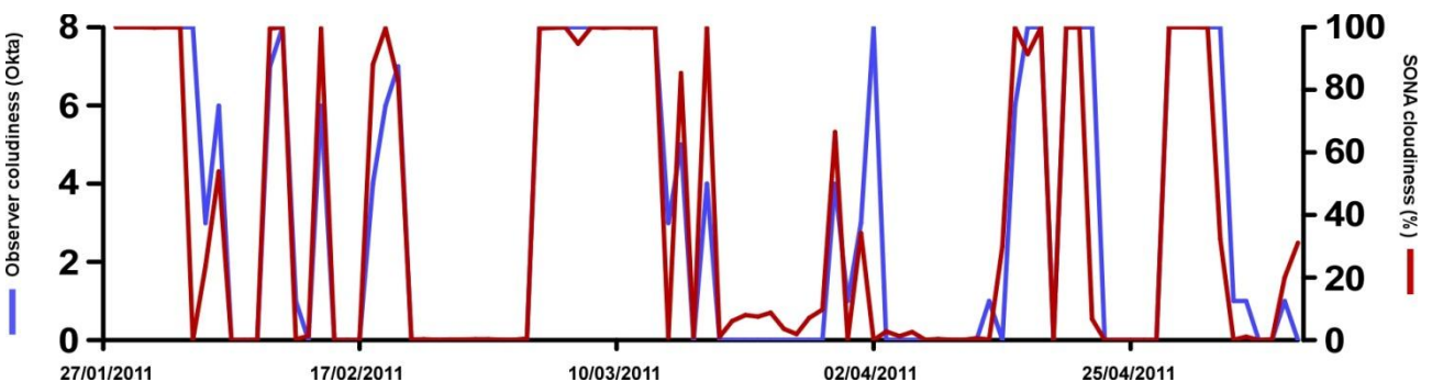
Fig.6 Cloudiness measured by observers (blue) by SONA (red). It exists a correlation between both data. Data from observes only can take eight different values (Okta), what makes the measures are less accurate.
