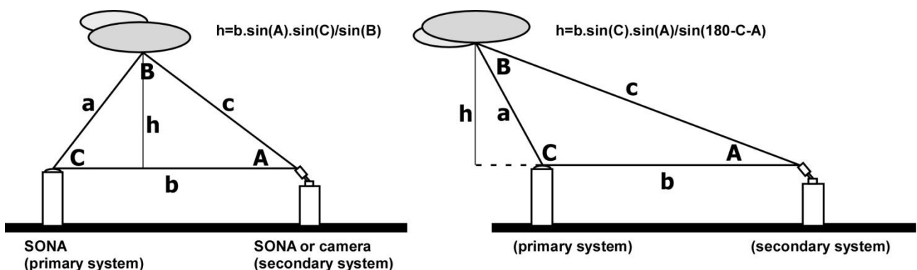
Fig.8 Cloud-base height estimation by triangulation. radiative transfer models of radiation
