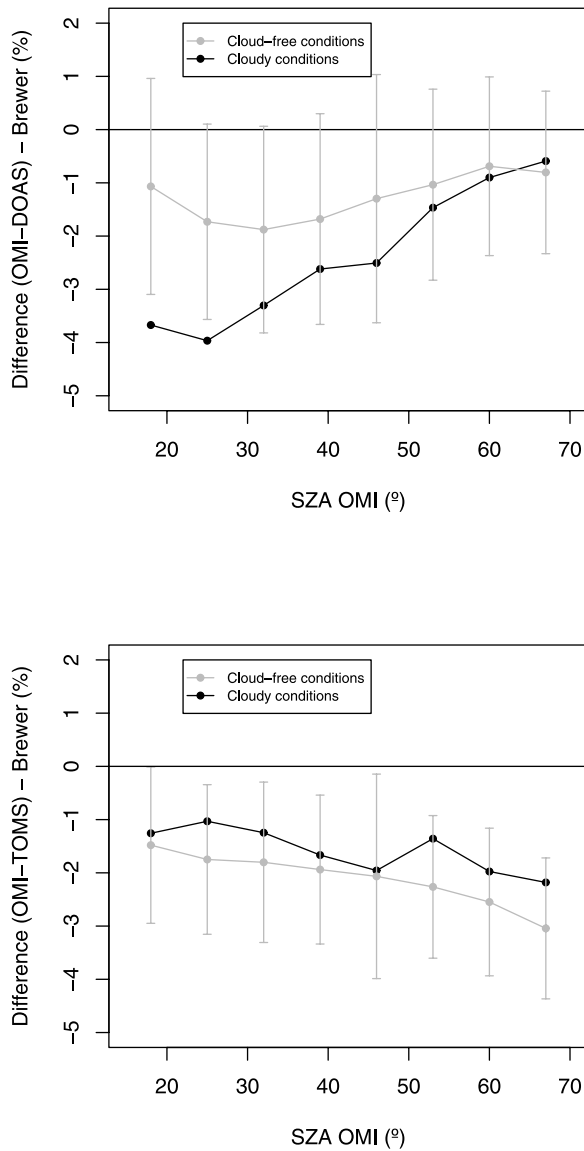
Figure 6. (top) Evolution of the differences between total ozone column data retrieved by OMI-DOAS and Brewer total ozone column data as function of solar zenith angle for cloud-free and cloudy conditions. (bottom) Evolution of the differences between total ozone column data retrieved by OMI-TOMS and Brewer total ozone column data as function of solar zenith angle for cloud-free and cloudy conditions.
