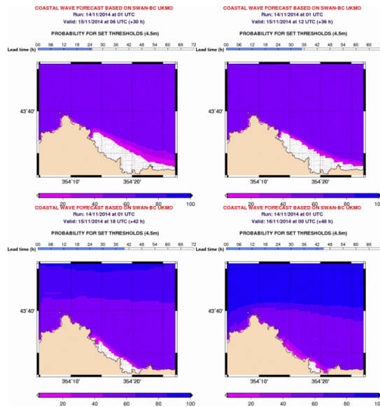
Fig 18 – Gijon probability maps. Hs threshold: 4.5 meters
