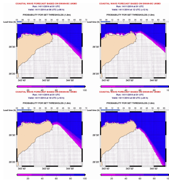
Fig 20 – Tenerife probability maps. Hs threshold: 1.8m
