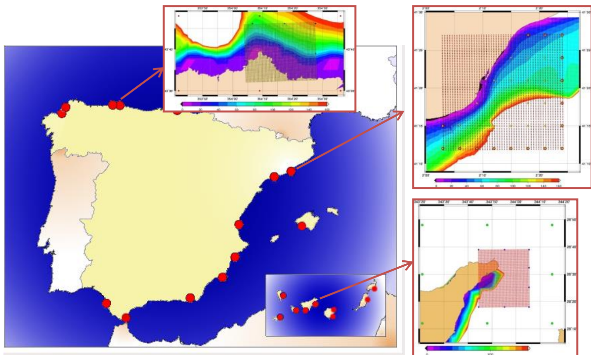
Figure 1 - Local wave forecast system for Spanish harbours operated by PdE (red points). In the boxes, new ensemble applications: Barcelona, Gijón and Tenerife.
