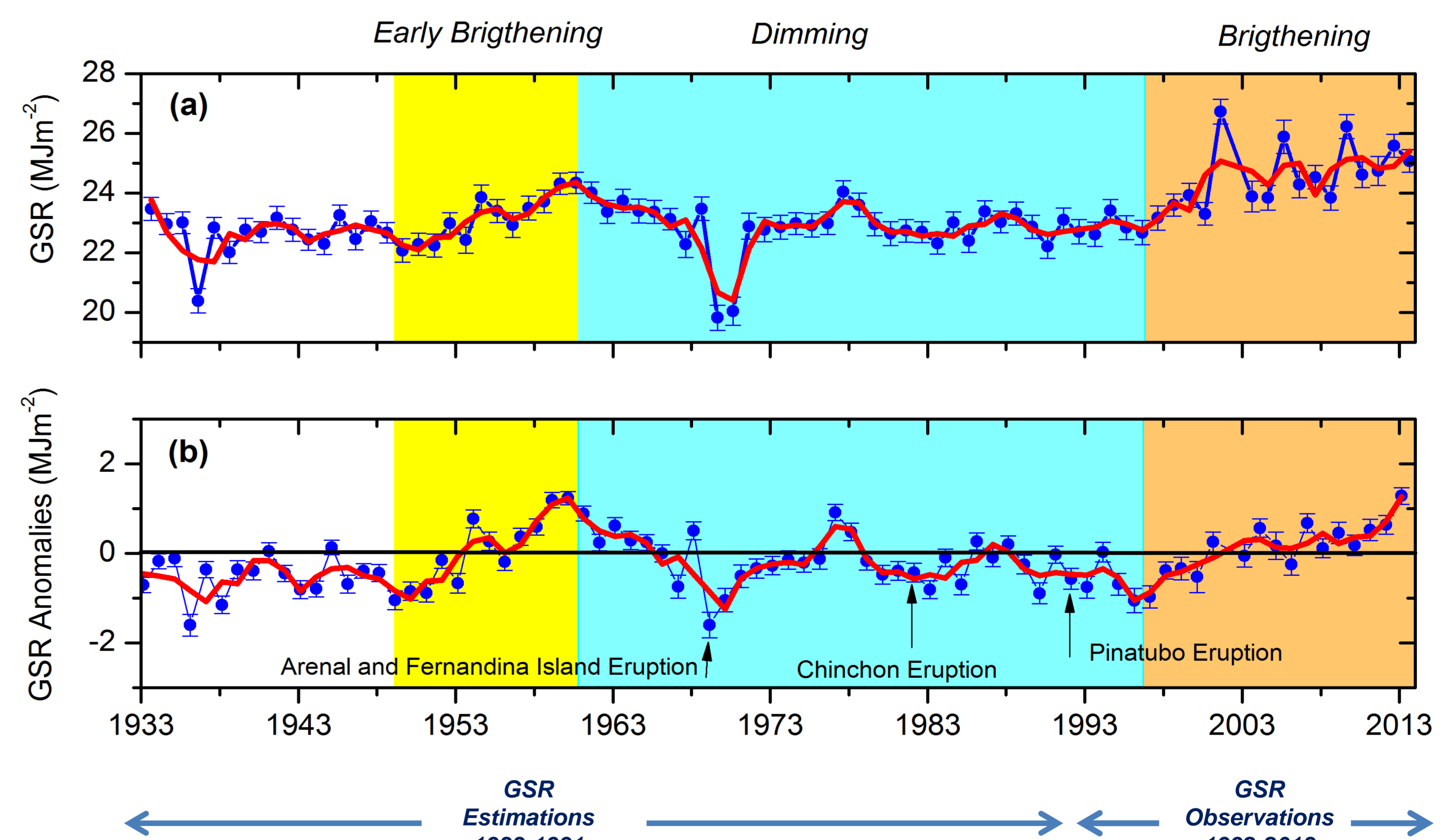
Figure 4.- Time series of the annual means of (a) GSR and (b) GSR anomalies from 1933 to 2013 at IZA. The error bars indicate \pm 1 SEM (standard error of the mean). The arrows indicate the eruptions of Arenal and Fernandina (1968), Chinchón (1982) and Pinatubo (1991). Five-yr moving average is shown in red. (Time series has been deseasonalised by subtracting the averaged GSR annual cycle, obtaining the annual mean anomalies time series).
