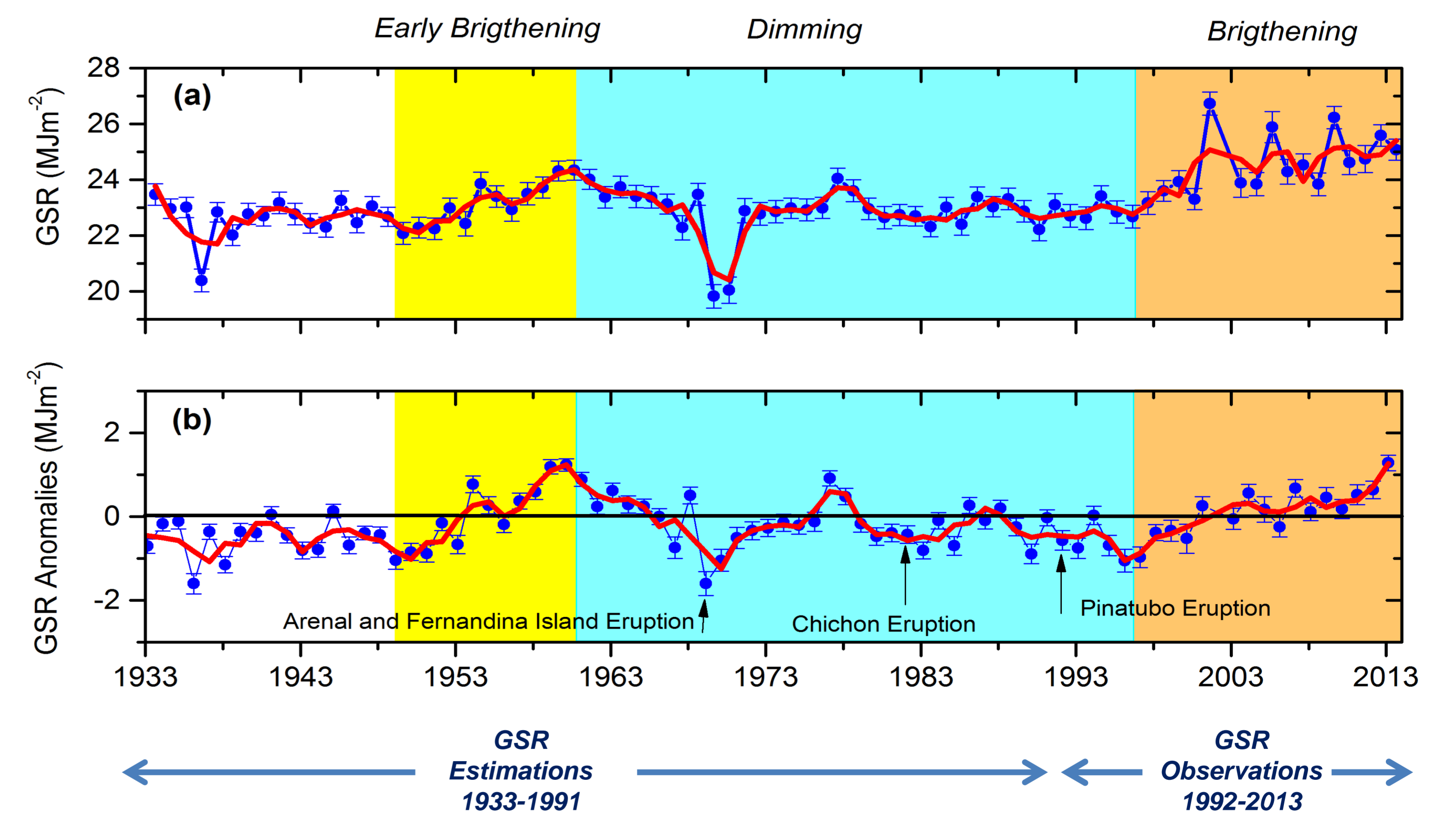
Figure 4.- Time series of the annual means of the (a) GSR and (b) GSR anomalies from 1933 to 2013 at IZA. The error bars indicate \pm 1 SEM (standard error of the mean) The arrows indicate the eruptions of Arenal and Fernandina (1968), Chichón (1982) and Pinatubo (1991). Five-yr moving average is shown in red. Time series has been deseasonalised by subtracting the averaged GSR annual cycle, obtaining the annual mean anomalies time series.
