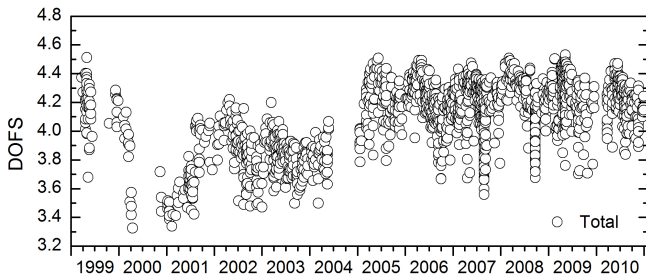
Fig. 3. Time series of total DOFS of retrieved ozone values using the setup C for the whole FTIR time series between 1999 and 2010 (number of data, N , is 1887).
