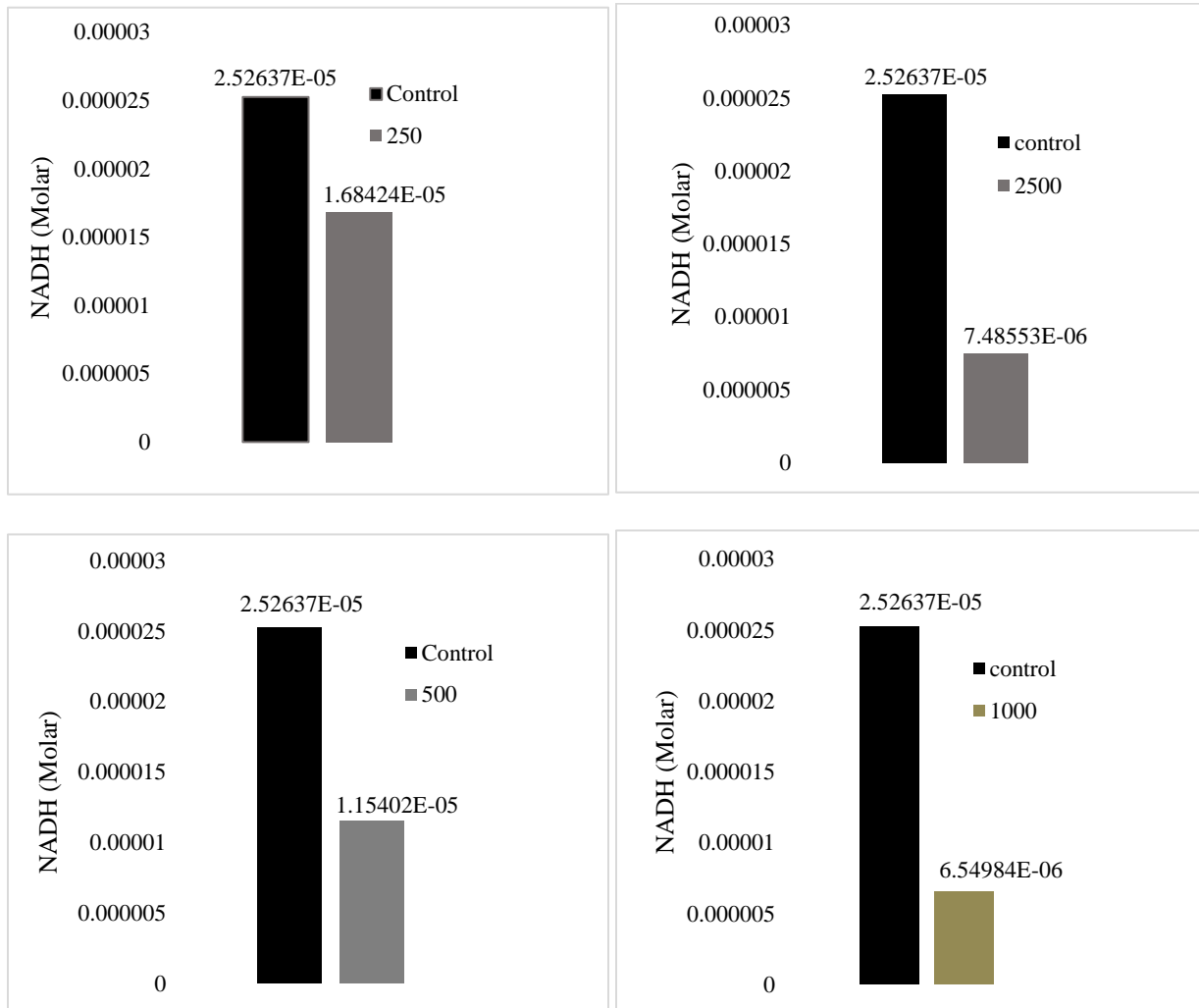
Figure 9. Average NADH conversion to NAD + per concentration of metformin.
