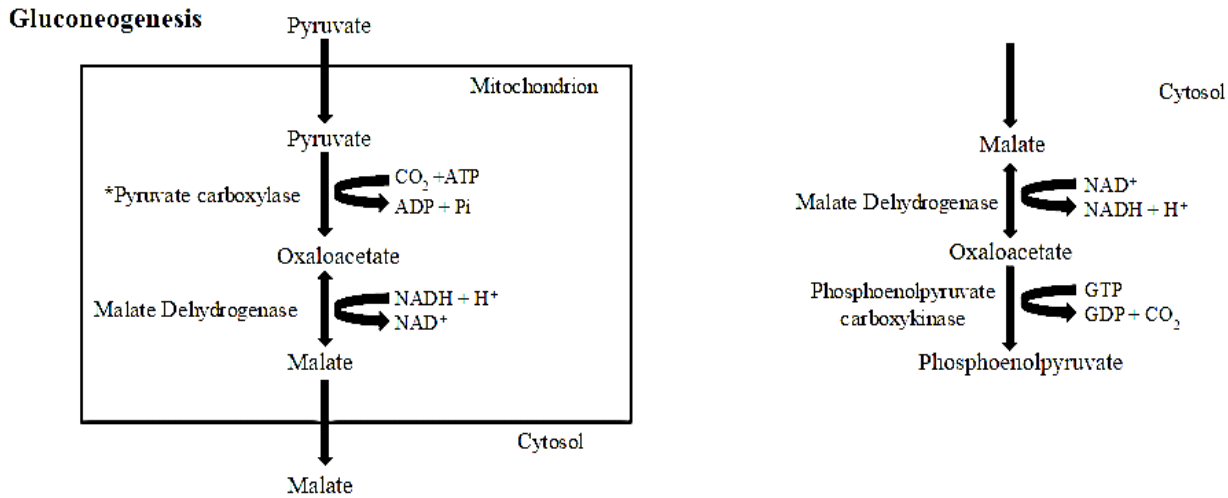
Figure 2. The pathway for mitochondrial gluconeogenesis is enzyme coupled in nature. Pyruvate carboxylase catalyzes the first step and Malate Dehydrogenase the second. From “Gluconeogenesis for medical school,” by R.,Kiran. http://www.slideshare.net/ravikiran35977897/gluconeogenesis-for-medical-school .
