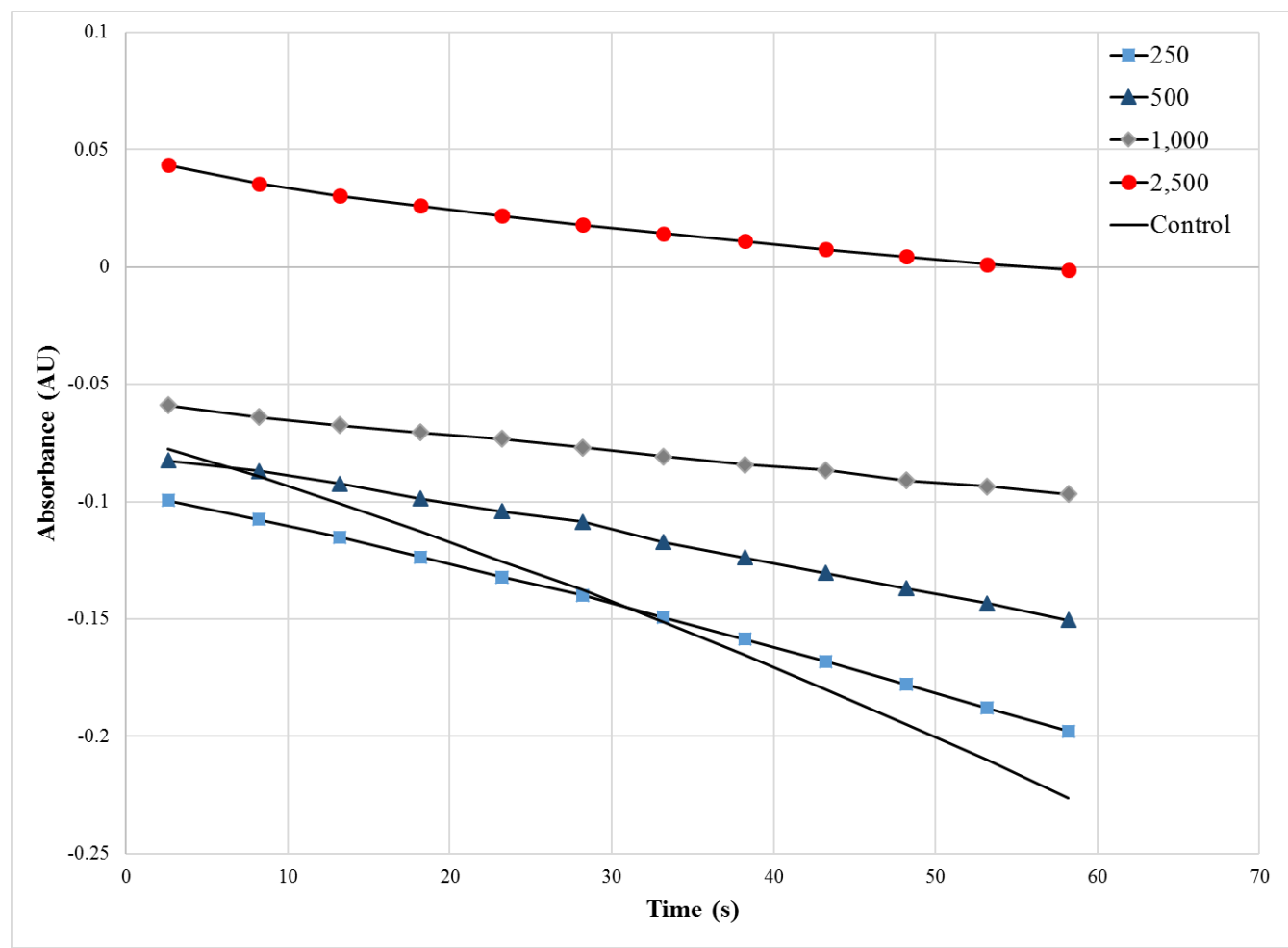
Figure 8. Graphical representation of the average rates (mol/sec) of the enzyme-coupled reactions treated with 250 \mu M-2,500 \mu M of metformin plus the controls are shown above. Significant differences between 500 \mu M, 1,000 \mu M and 2,500 \mu M were found.
