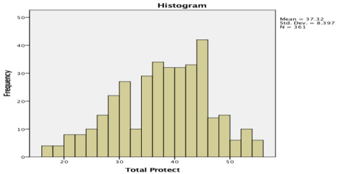
Figure 7. Normally distributed histogram for protect.
