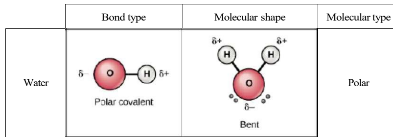
Figure 8.1: Polarity of the water molecule due to the uneven distribution of electrons in its covalent bond. C (From OpenStax Concepts of Biology text)
