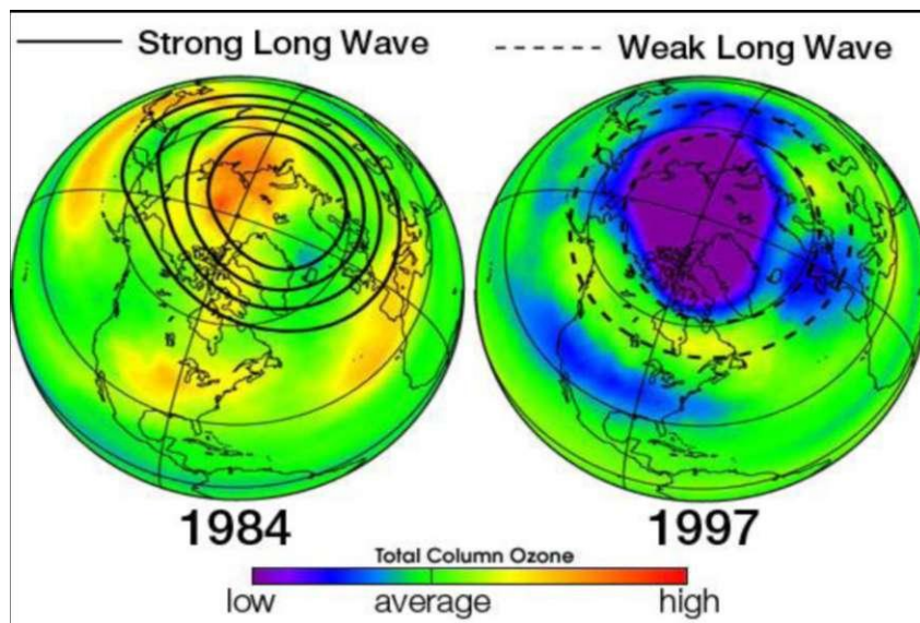
Figure 6.6: Seasonal ozone depletion over North America was lower in 1984 and greater in 1997. source: NASA http://earthobservatory.nasa.gov/IOTD/view.php?id=1771
