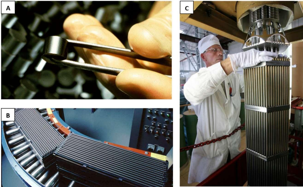
Figure 4.14: Fuel fabrication process. A) Uranium dioxide powder compressed into fuel pellets . B) Fuel pellets stacked and sealed in metal tubes forming rods . C) Fuel rods are bundled into a fuel assembly . Images A and B from NRC (public domain); C from RIA Novosti archive, image #132602 / Ruslan Krivobok / CC-BY-SA 3.0
