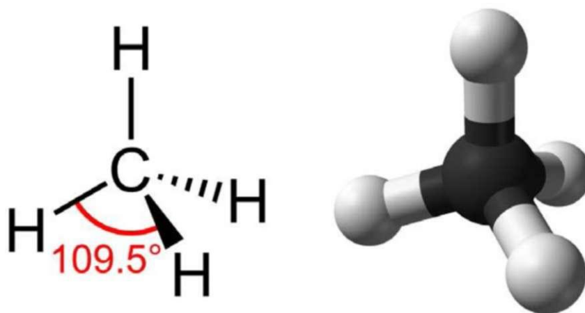
Figure 1.2. Methane (CH 4 ) has a tetrahedral geometry, with each of the four hydrogen atoms spaced 109.5° apart.
