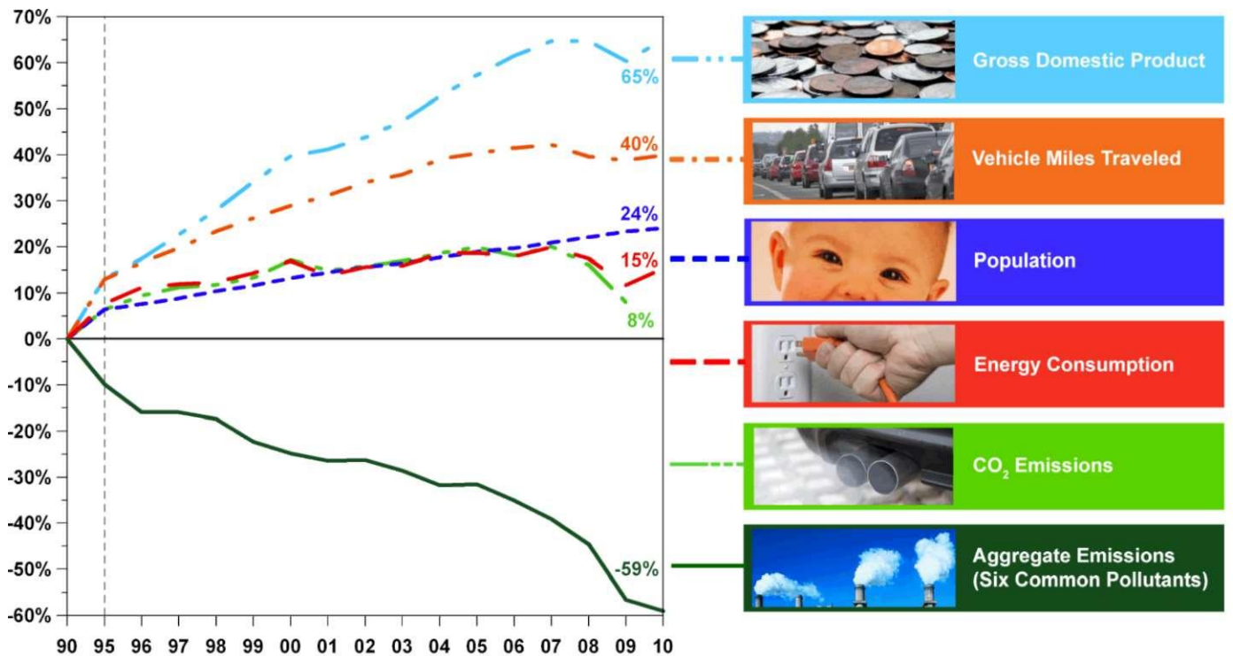
Figure 6.14: Showing a decrease in the combined emissions for the six criterial pollutants in the past two decades. Meanwhile, population, energy consumption, vehicle miles travelled, and gross domestic product have all increased. Source: US EPA
