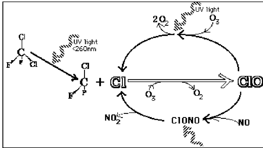
Figure 6.5: Ozone destruction. UV radiation frees a chlorine (Cl) atom from a CFC molecule, this atom reacts with ozone and produces an oxygen gas molecule and chlorine monoxide (ClO). ClO reacts with another oxygen atom, it frees up the Cl atom which then proceeds to destroy another ozone molecule. source: Wiki commons https://commons.wikimedia.org/wiki/Category:Ozone#/media/File:Chlorine_catalysis.GIF
