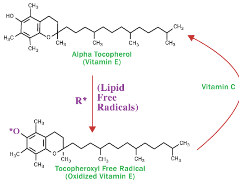
Figure 9.23 Conversion of alpha-tocopherol to alpha-tocopherol radical 2
