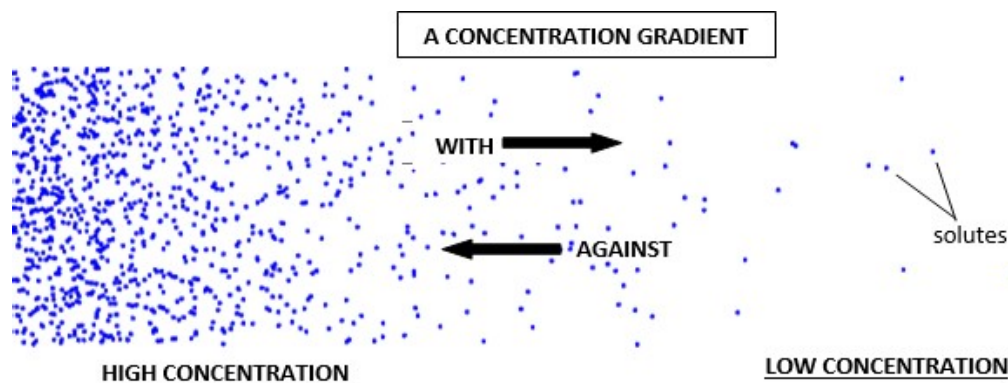
Figure 4.31 Movement with and against a concentration gradient.
