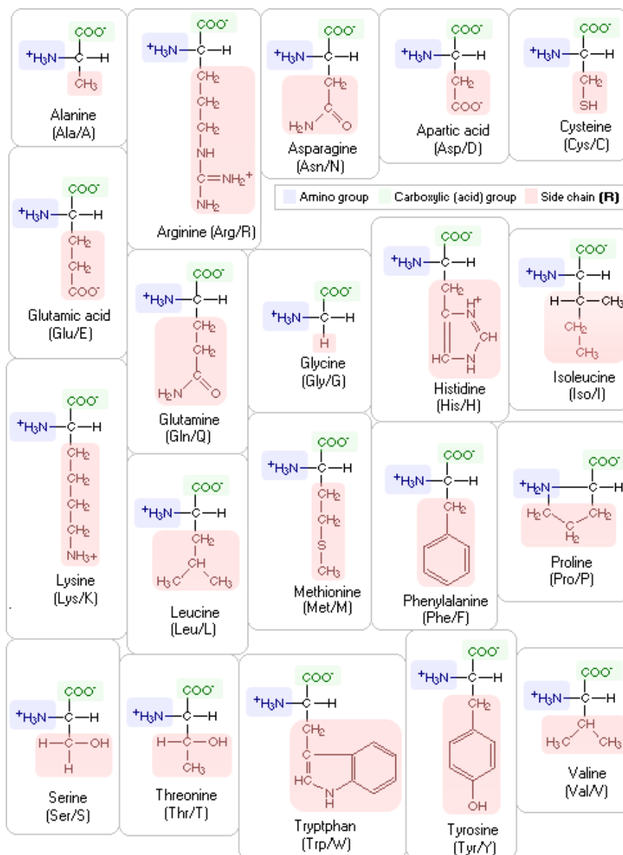
Figure 2.262 Amino acid structures for the 20 amino acids found in the human body 1
