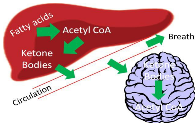
Figure 6.342 The production, release, use, or exhalation of ketone bodies 2
