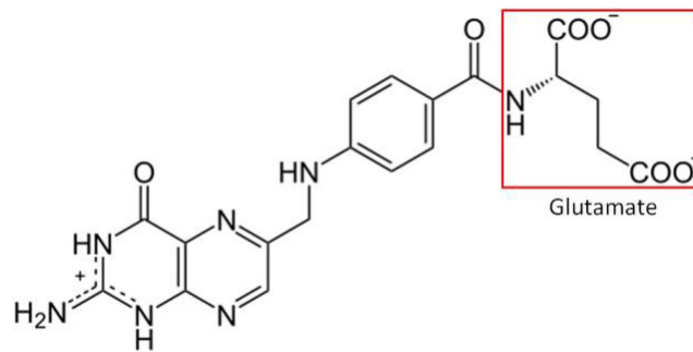
Figure 11.11 Structure of Folic Acid 1
