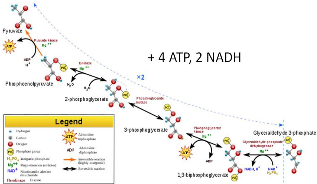
Figure 6.235 Glycolysis step 3, energy harvesting 1
