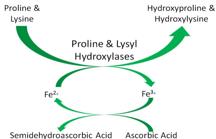
Figure 12.732 Importance of ascorbic acid and iron to proline and lysyl hydroxylases.
