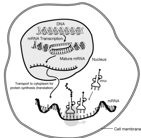
Figure 2.221 The process of creating a polypeptide 1
