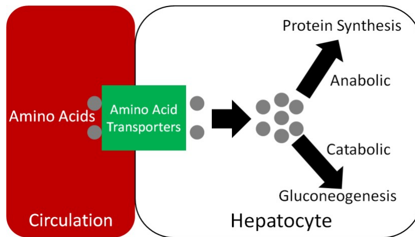
Figure 4.64 Hepatic amino acid uptake
