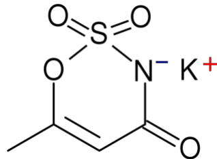
Figure 2.135 Structure of acesulfame-potassium (K) 9
