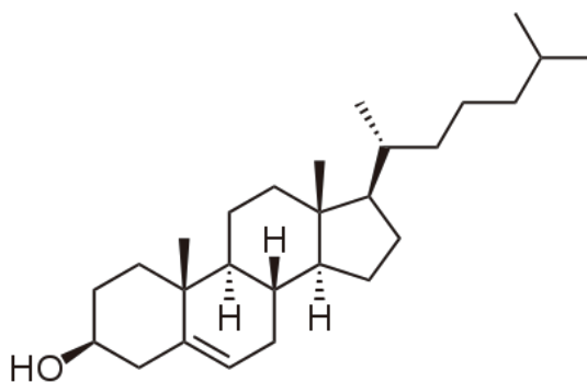
Figure 2.372 The carbon ring structure of cholesterol 1
