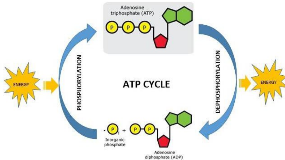
Figure 4.34 The ATP Cycle demonstrating the processes of phosphorylation and dephosphorylation.
