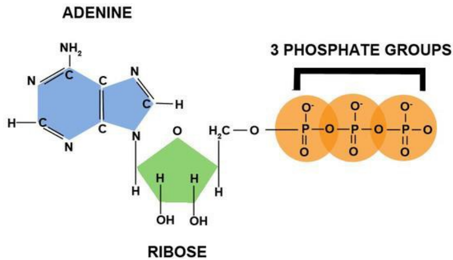
Figure 4.33 Structure of adenosine triphosphate (ATP) 1
