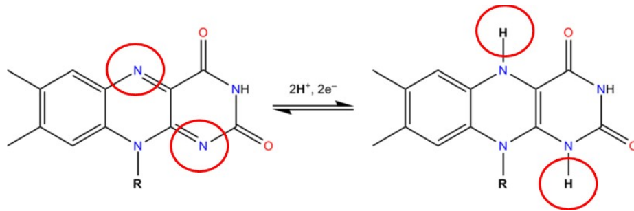
Figure 6.112 The reduction of FAD (left) to FADH 2 (right) 4
