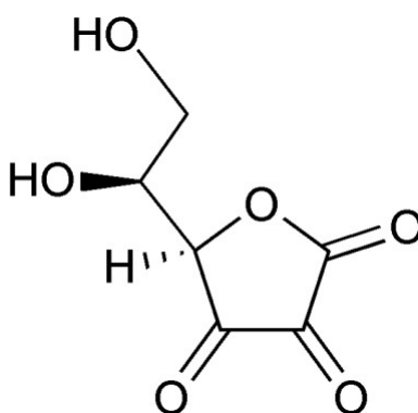
Figure 9.32 Structure of dehydroascorbic acid 3 . Notice the change in the two bottom OH groups from Figure 9.31.
