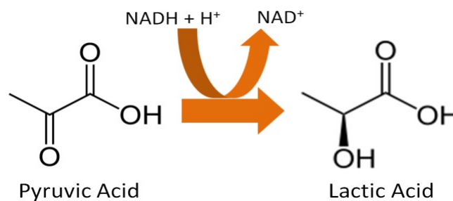
Figure 6.283. The conversion of pyruvic acid to lactic acid regenerates NAD 3,4
