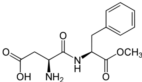
Figure 2.132 Structure of aspartame 6
