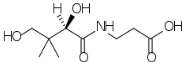
Figure 10.61 The structure of pantothenic acid 1
