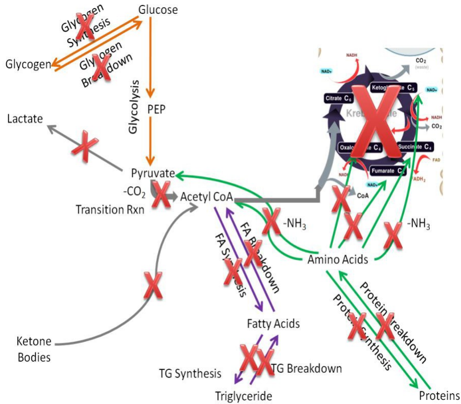
Figure 7.342 The metabolic pathways that are not performed or important in the red blood cells, compared to extrahepatic tissues as a whole are crossed off 2
