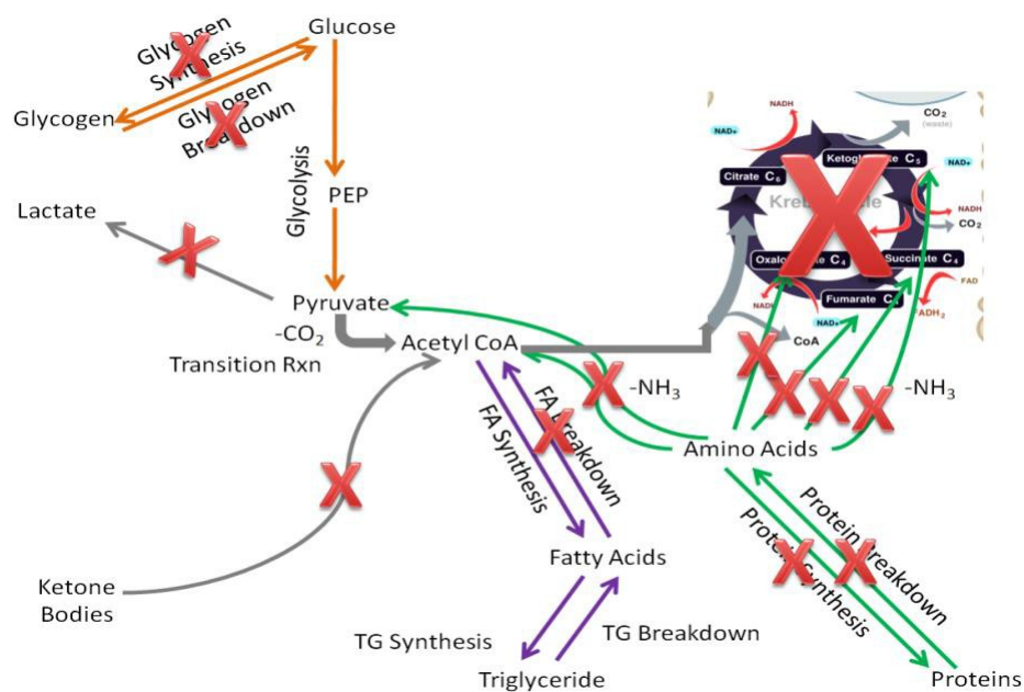
Figure 7.321 The metabolic pathways that are not performed or important in adipose tissue, compared to extrahepatic tissues as a whole are crossed out 1
