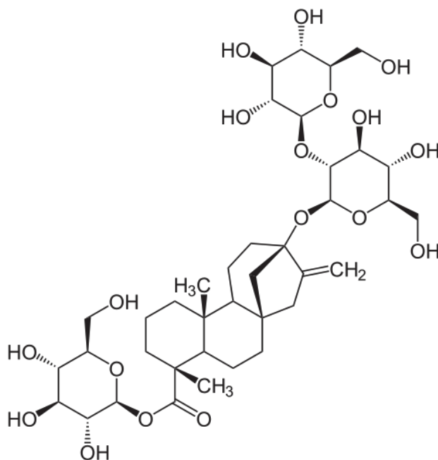
Figure 2.138 Structure of stevioside 14
