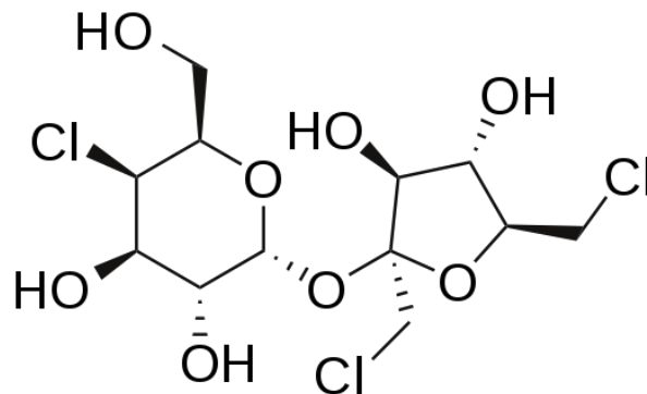
Figure 2.136 Structure of sucralose 10
