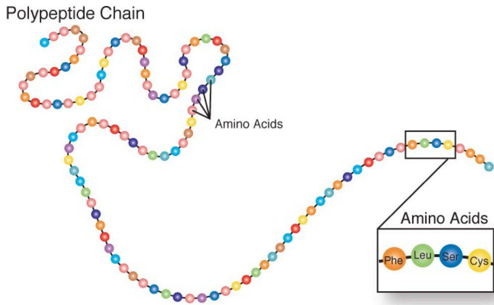
Figure 2.216 A polypeptide chain 2
