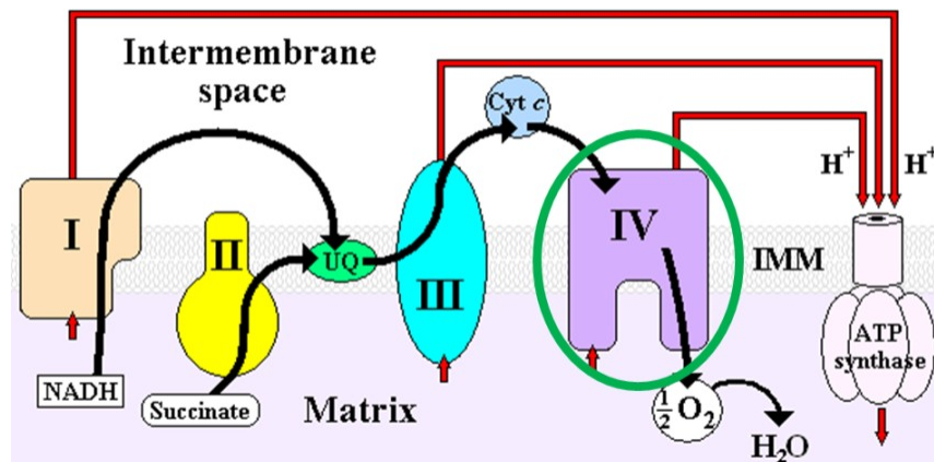
Figure 12.915 Cytochrome c oxidase (complex IV) 2
