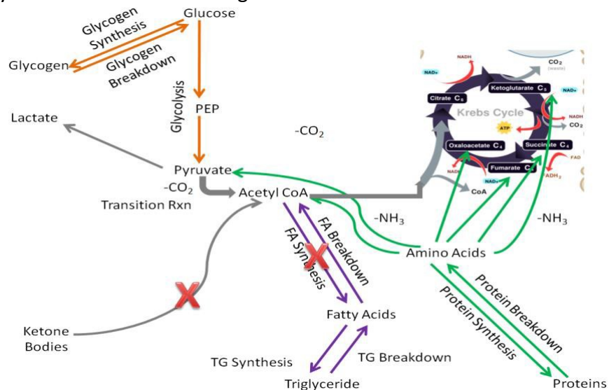
Figure 7.311 The metabolic pathways that are not performed or important in muscle tissue, compared to extrahepatic tissues as a whole 1
