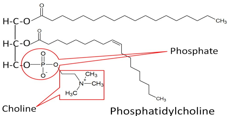
Figure 2.362 Structure of phosphatidylcholine (lecithin)
