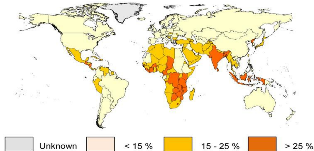
Figure 12.821 Worldwide prevalence of zinc deficiency 1
