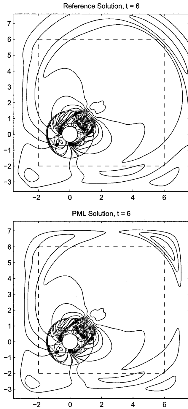
FIG. 20: Transient pressure pulse: Contours of density at time t = 6 .
