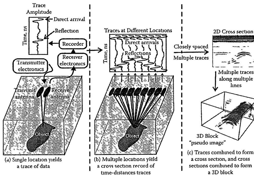
FIG. 21. Process for using ground-penetrating radar to construct a 3-dimensional pseudo-image of a buried object. From Daniels et al. (2008).
