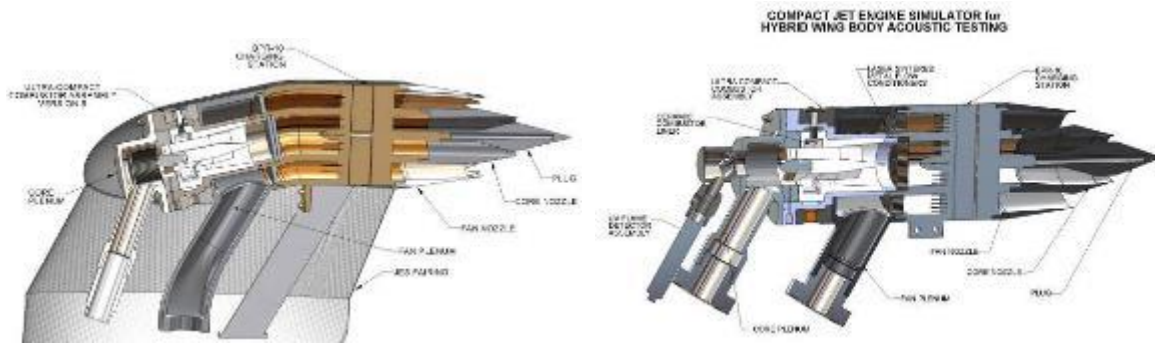
Figure B-4 Compact Jet Engine Simulator Variations before Detail Design Contract. (5)
