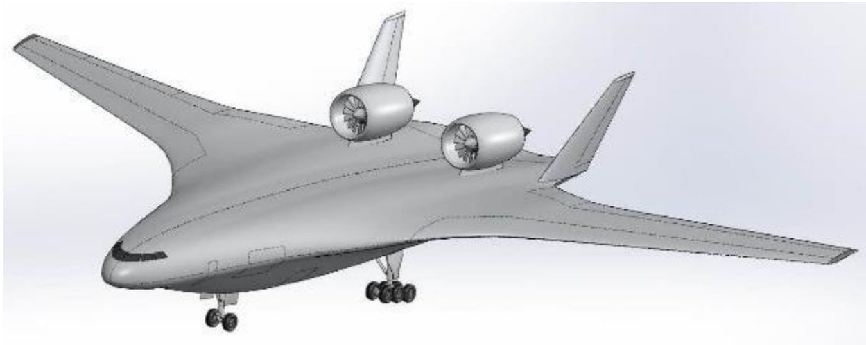
Figure 11. Boeing Concept of the Hybrid Wing Body Aircraft. (5)
