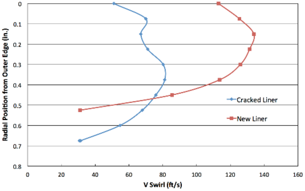
Figure 31 Swirl Air Velocity in the Combustor Annulus. (36)
