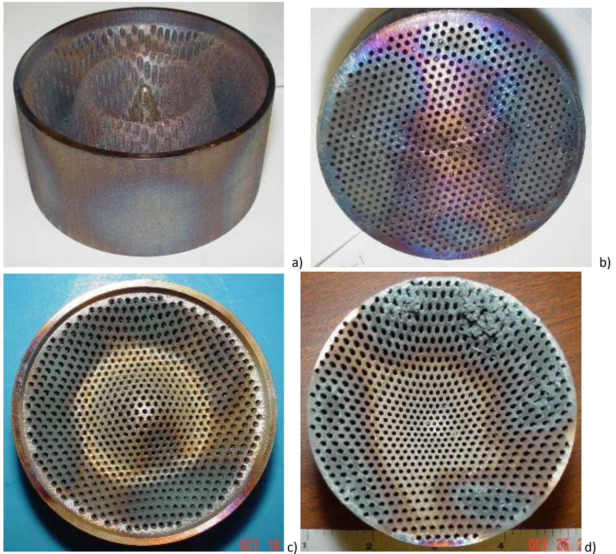
Figure 50 Core Flow Conditioners Exhibiting Nonuniform Heating. Pictures a) and b) show upstream and downstream view of the same part, c) shows a Single Sinusoid, d) shows a Concave Unit. (12)
