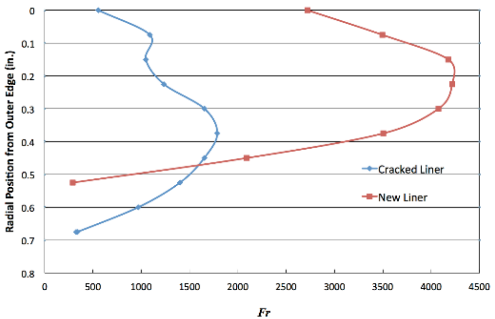
Figure 32 Froude Number for Cracked and New Combustor Liners. (36)
