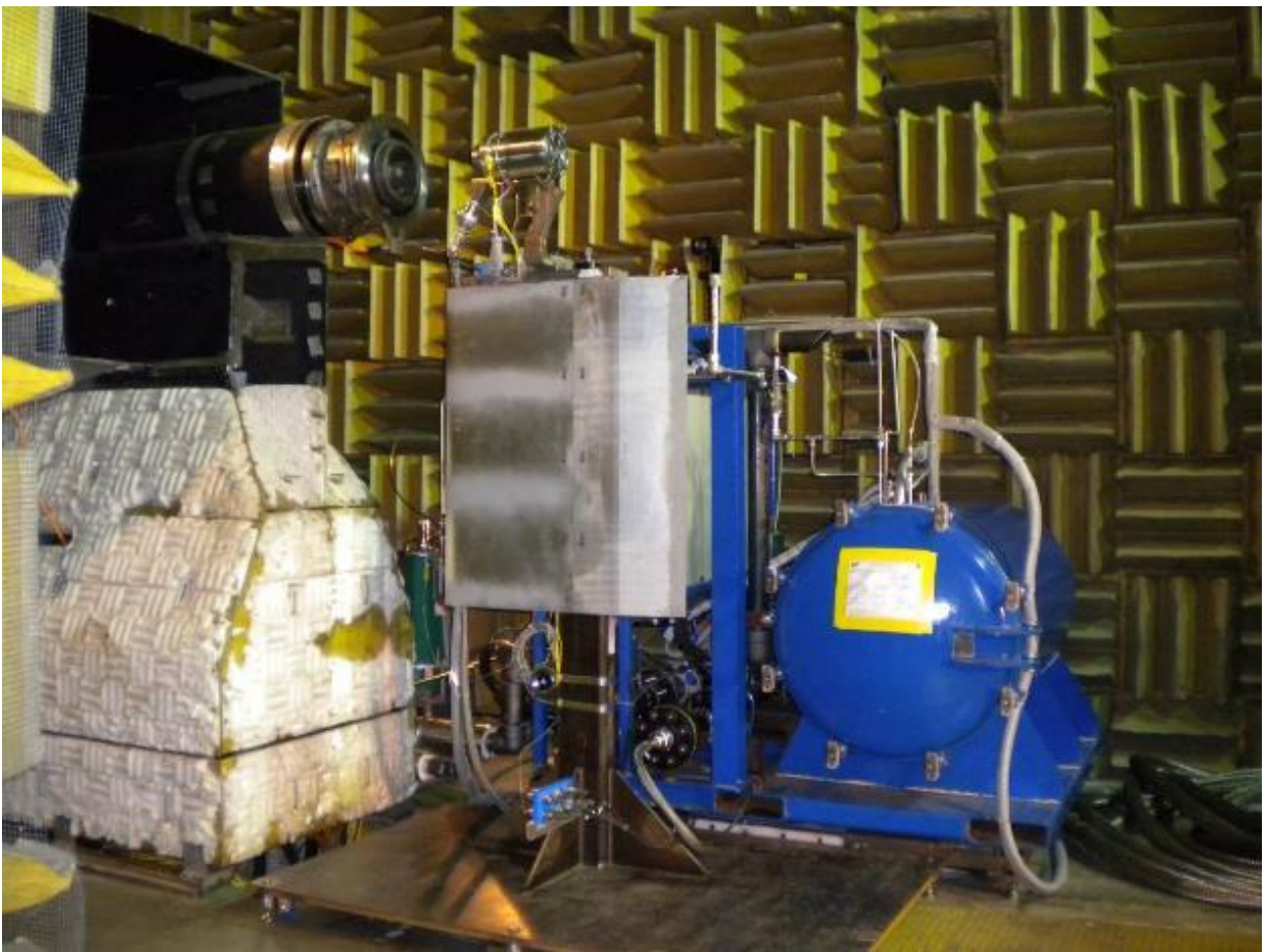
Figure 28 Initial testing Configuration of CJES Combustor in the Jet Noise Laboratory. (12)
