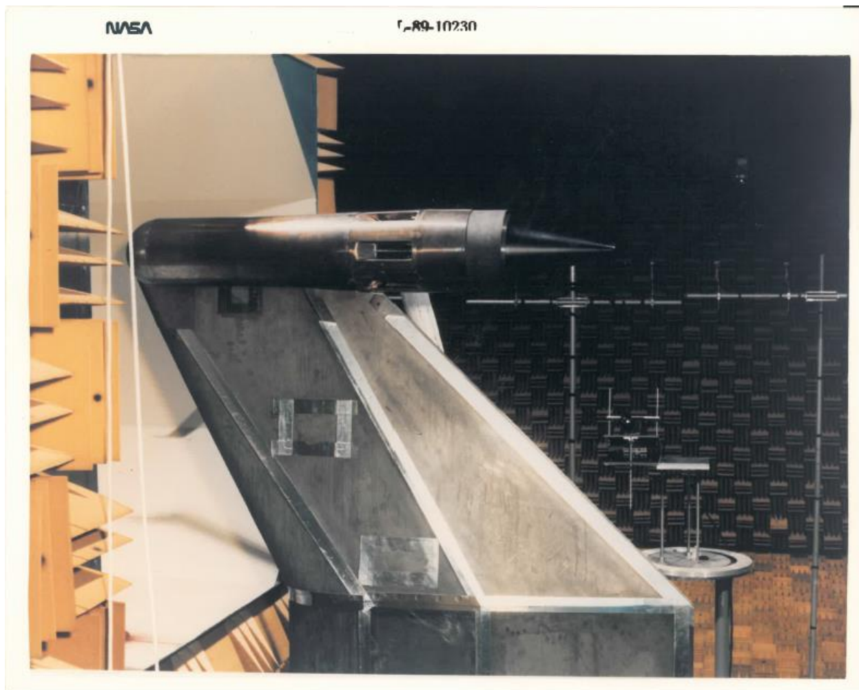
Figure 4 Boeing Nozzle Test Rig in 1989, (NASA photo L-89-10230)
