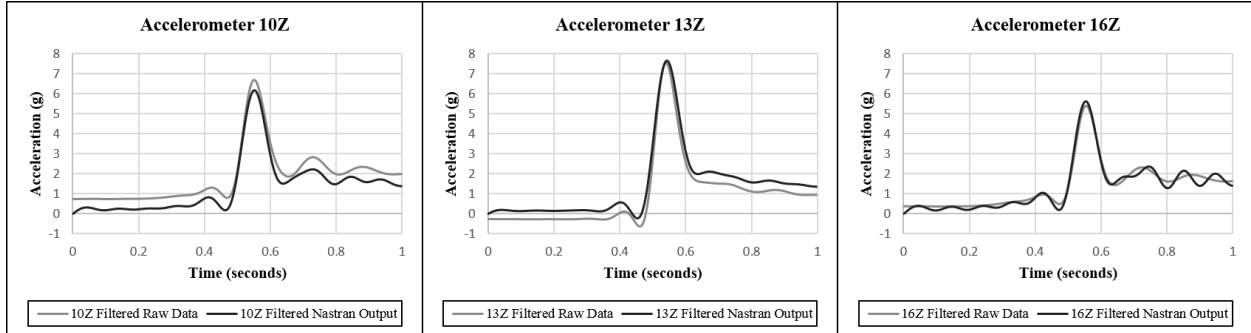
(a) Filtered Subcase 1 of Maximum Safe Speed Envelope. Average Craft Speed 19.0 knots. Significant Wave Height 5.0 feet. Average Wave Period 6.2 seconds.
