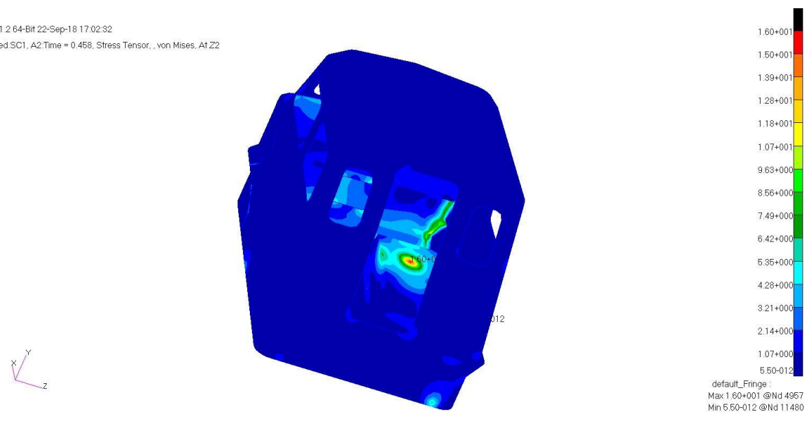
Figure 27. Cabin Stress Contour Plot at Z2: Starboard Seat Pedestal Node 4957
