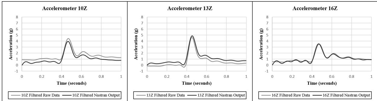
(c) Filtered Subcase 3 of Maximum Safe Speed Envelope. Average Craft Speed 30.4 knots. Significant Wave Height 3.4 feet. Average Wave Period 6.4 seconds.
