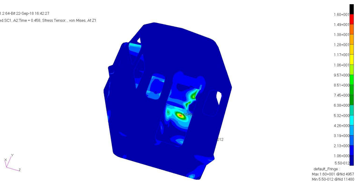
Figure 28. Cabin Stress Contour Plot at Z1: Starboard Seat Pedestal Node 4957
