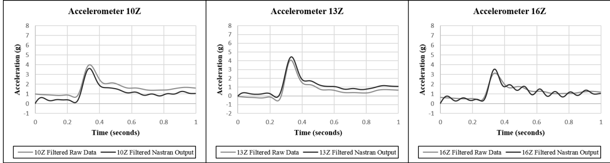
(b) Filtered Subcase 2 of Maximum Safe Speed Envelope. Average Craft Speed 35.8 knots. Significant Wave Height 2.3 feet. Average Wave Period 7.5 seconds.
