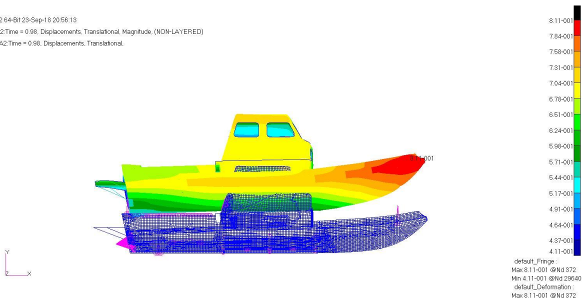
Figure C6. Side View of Deformation plot at 0.98 seconds
