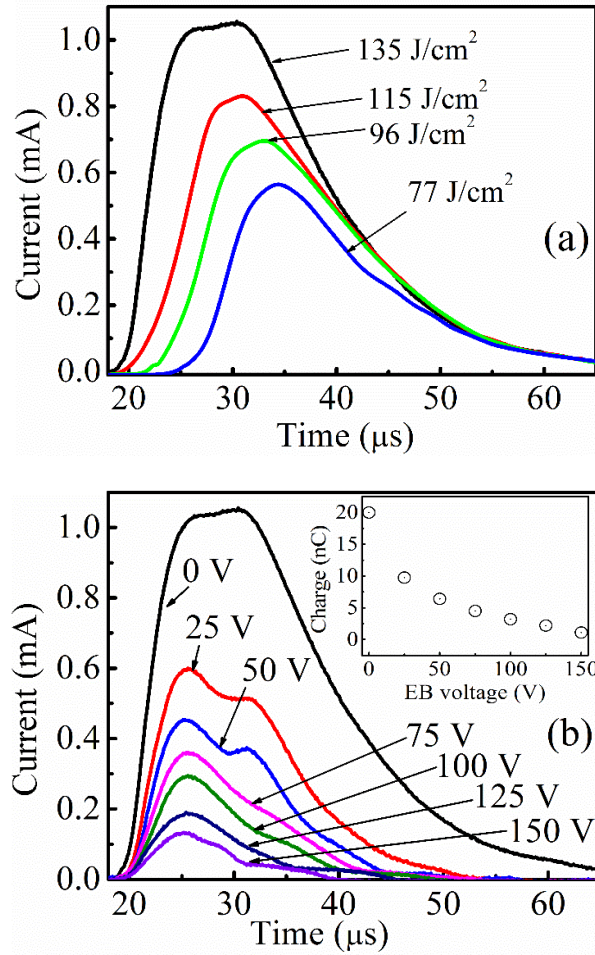
Fig. 7.3 (a) Ion signal detected by the FC-1 for increasing laser fluence. (b) Ion signal for a laser fluence of 135 \text{ J/cm}^2 with different applied barrier voltages. Inset shows the total charge detected with the increase of barrier voltage.
