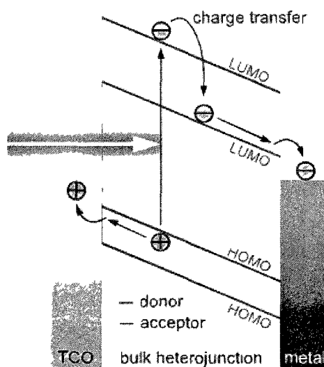
Figure II.4: Band bending in a bulk heterojunction solar cell; upon exciton dissociation, the bending of the LUMO and HOMO transport the charges to the electrodes
