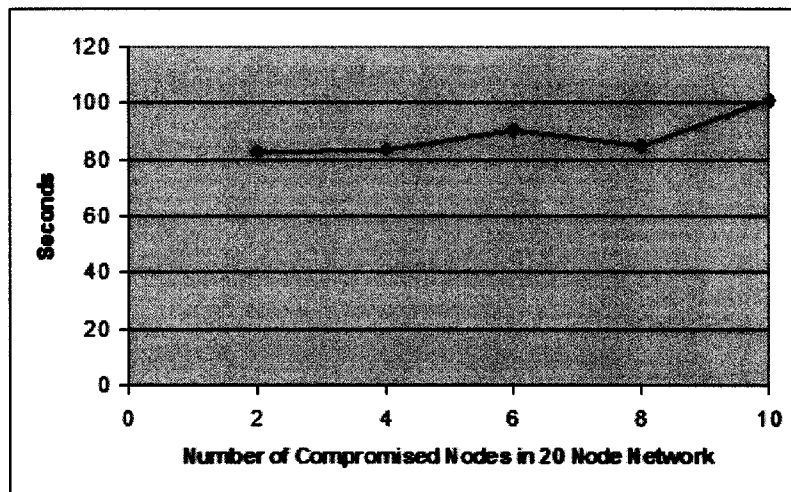
Figure 14. Average Time to Detect a Compromised Node in a 20 Node Network.
