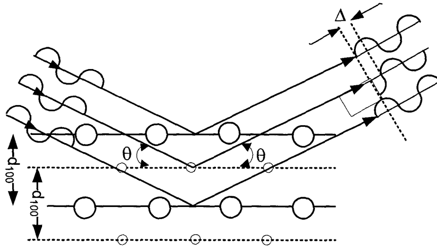
Fig. 2.3. The CsCl structure viewed along (100) plane. The scattered waves are in phase if they are scattered off the atoms of the same type. Destructive interference results from a phase difference of 2\pi\Delta/\lambda between the scattered waves from successive planes. Reproduced from Ref. [2].
