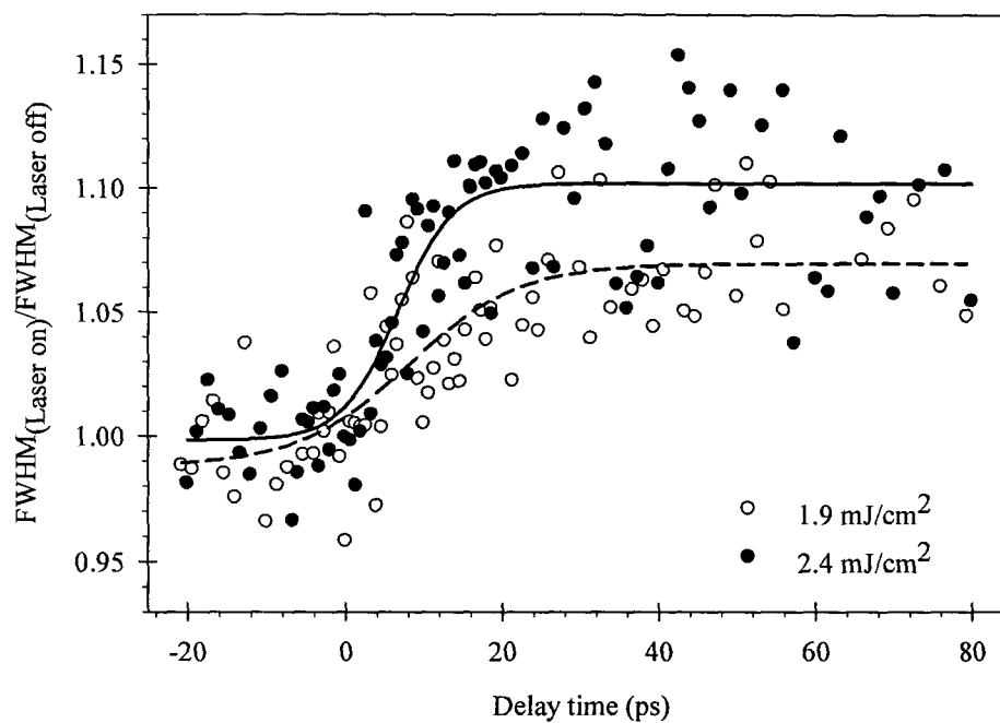
Fig. 7.9. Relative change in Bragg peak FWHM as a function of delay time of photoexcited Bi nanoclusters by laser fluence of 1.9 \text{ mJ/cm}^2 and 2.4 \text{ mJ/cm}^2 for (012) Bragg peak.
