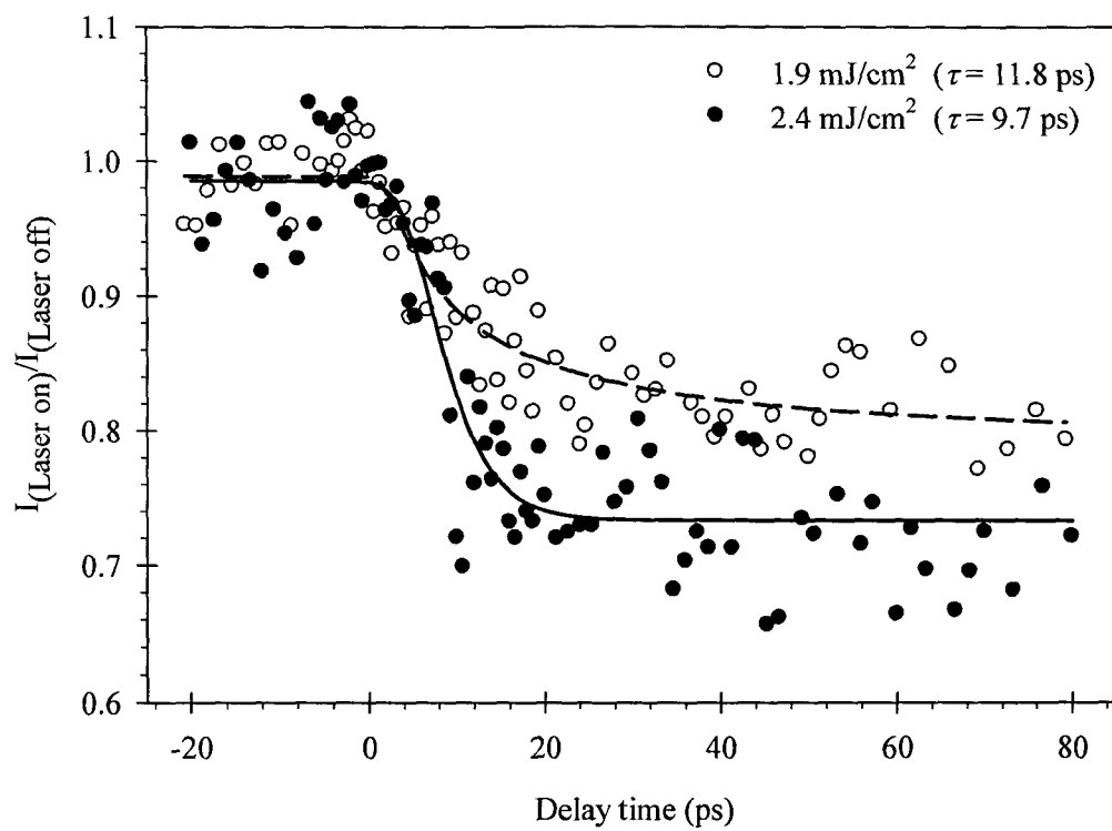
Fig. 7.4. Time dependent normalized intensity of Bragg peak (012) of photoexcited Bi nanoclusters by laser fluence of 1.9 mJ/cm 2 and 2.4 mJ/cm 2 .
