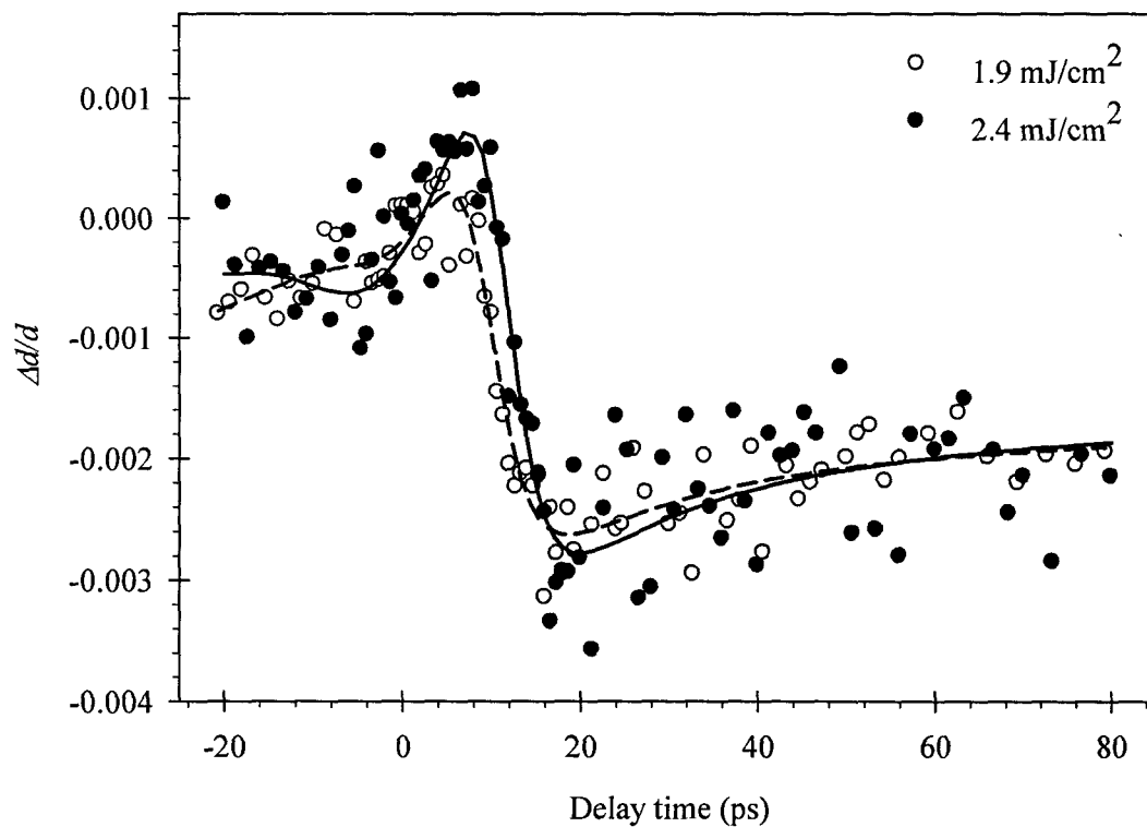
Fig. 7.7. Relative change in Bragg peak position ( \Delta d/d ) as a function of delay time for Bragg peak (012) of photoexcited Bi nanoclusters by laser fluence of 1.9 mJ/cm 2 and 2.4 mJ/cm 2 .
