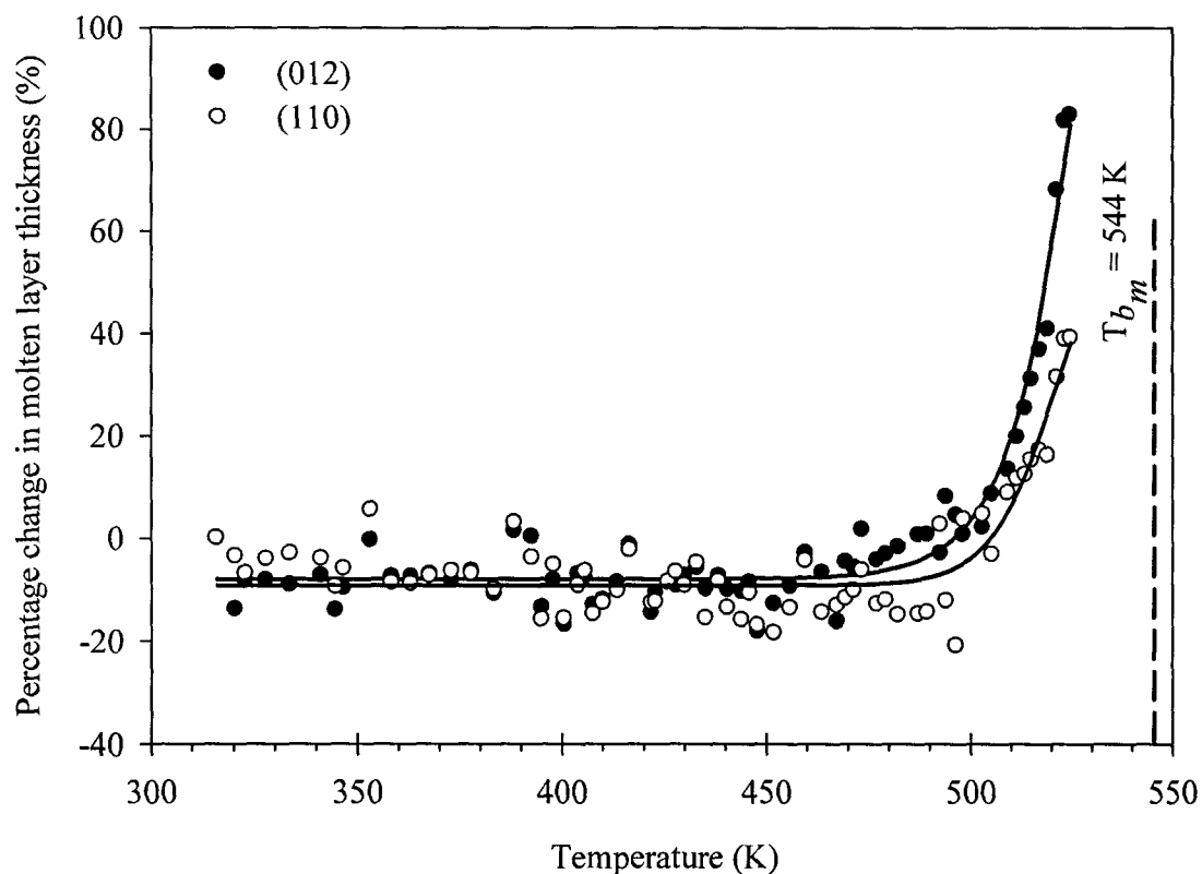
Fig. 5.8. Temperature dependence of the percentage change in the molten layer thickness, calculated from diffraction ring FWHM at temperature T normalized to that at temperature T = 323 K.
