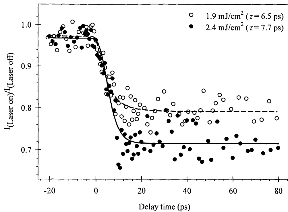
Fig. 7.5. Time dependent normalized intensity of Bragg peak (110) of photoexcited Bi nanoclusters by laser fluence of 1.9 mJ/cm 2 and 2.4 mJ/cm 2 .
