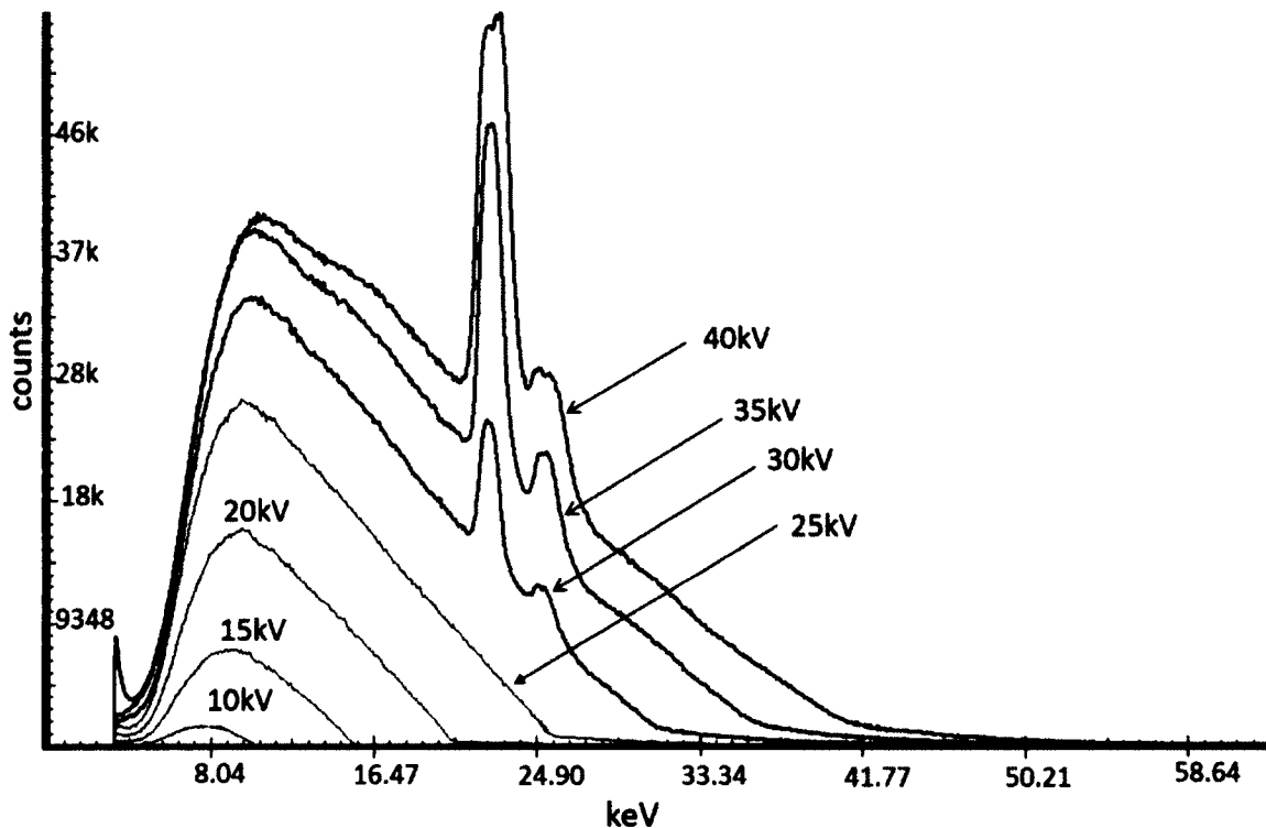
Figure 14. Tube characterization photon count curves from 10 kV to 40 kV in 5 kV increments. The energy scale was calibrated with a 1 micro Currie Am-241 source.
