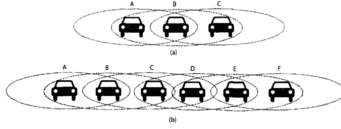
Fig. 14: GVC Hidden terminal discovery.
