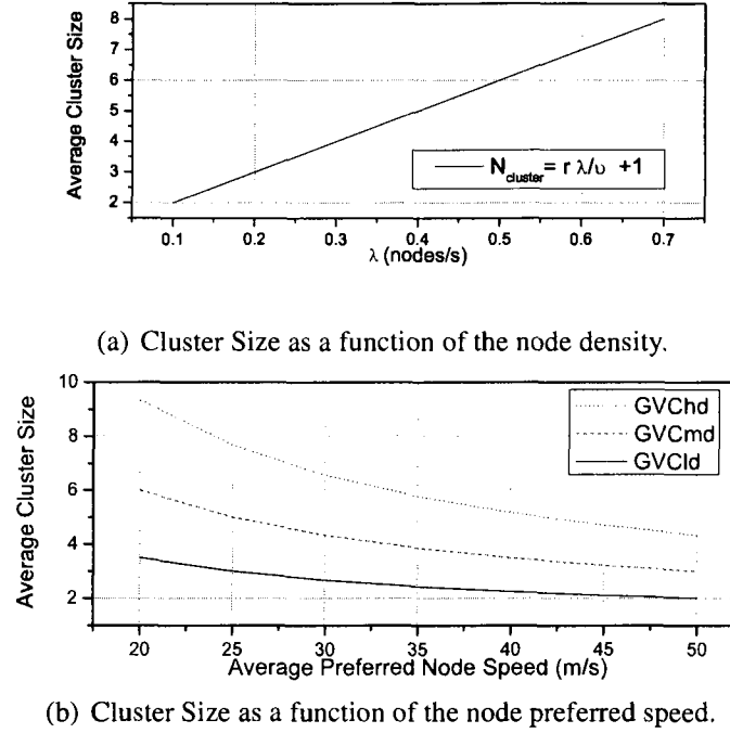
Fig. 15: The model of the average cluster size.
