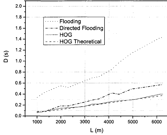
Fig. 28: Delay for R = 450 m.
