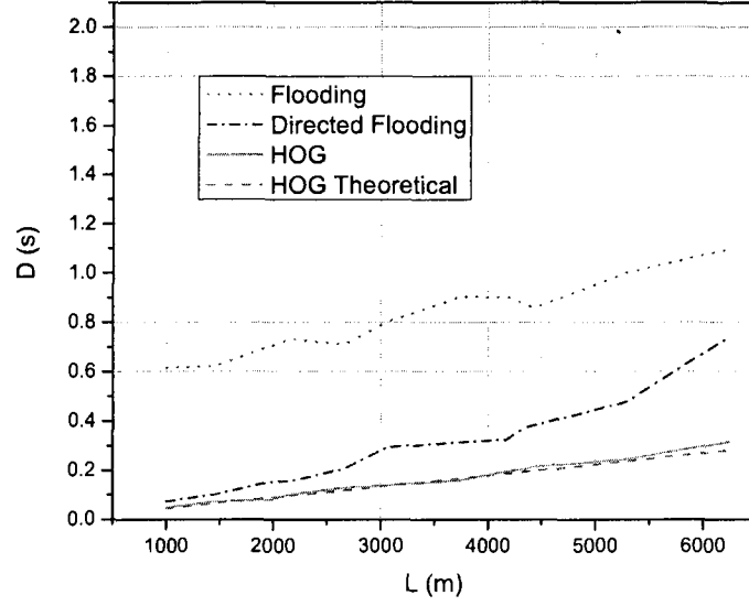
Fig. 29: Delay for R = 600 m.
