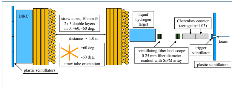
Figure 2. Sketch of the detection system for the follow-up experiment.
