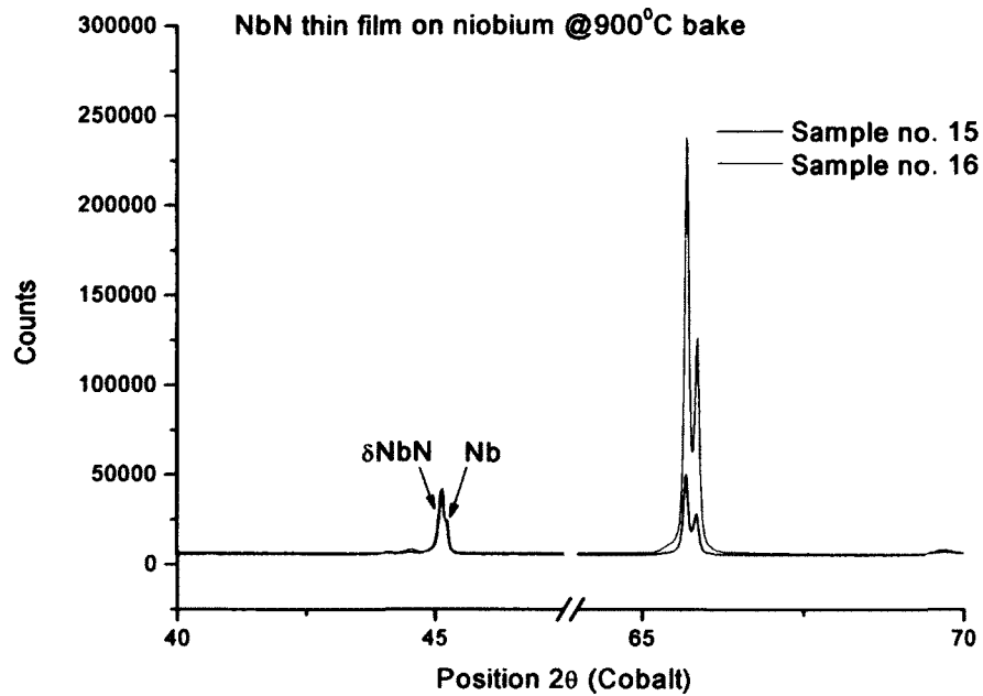
FIG. 32. XRD spectra showing the presence of presence of \delta\text{NbN} , Nb and \alpha\text{NbN} on niobium substrate.
