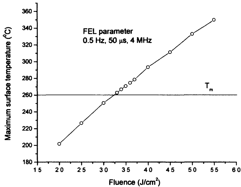
FIG. 51. Maximum surface temperature vs fluence
