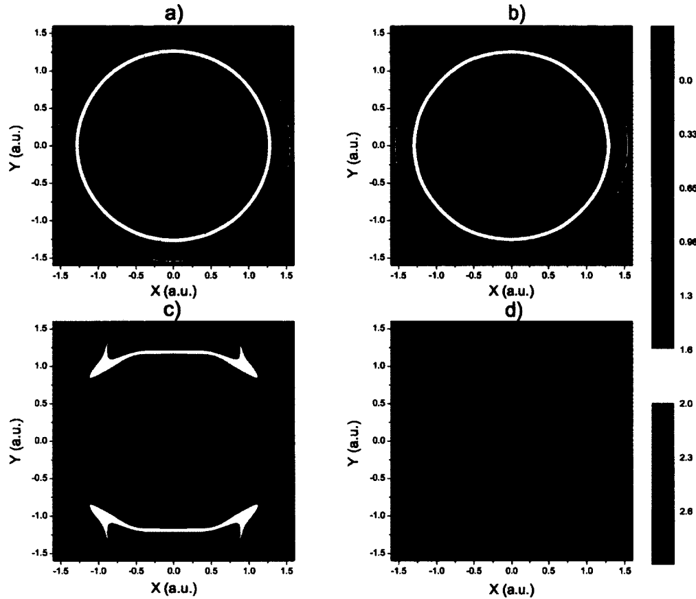
FIG. 50. The Inverse Radon transform of parabolic distribution function obtained using the filtered back projection method on the 0^{\circ} - 180^{\circ} range of angles at a) 17 projections on 45 angles, b) 17 projections on 21 angles, c) 17 projections on 5 angles, and d) 5 projections on 21 angles.
