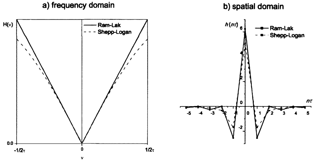
FIG. 46. Ram-Lak and Shepp-Logan filters in a) frequency and b) spatial domain.
