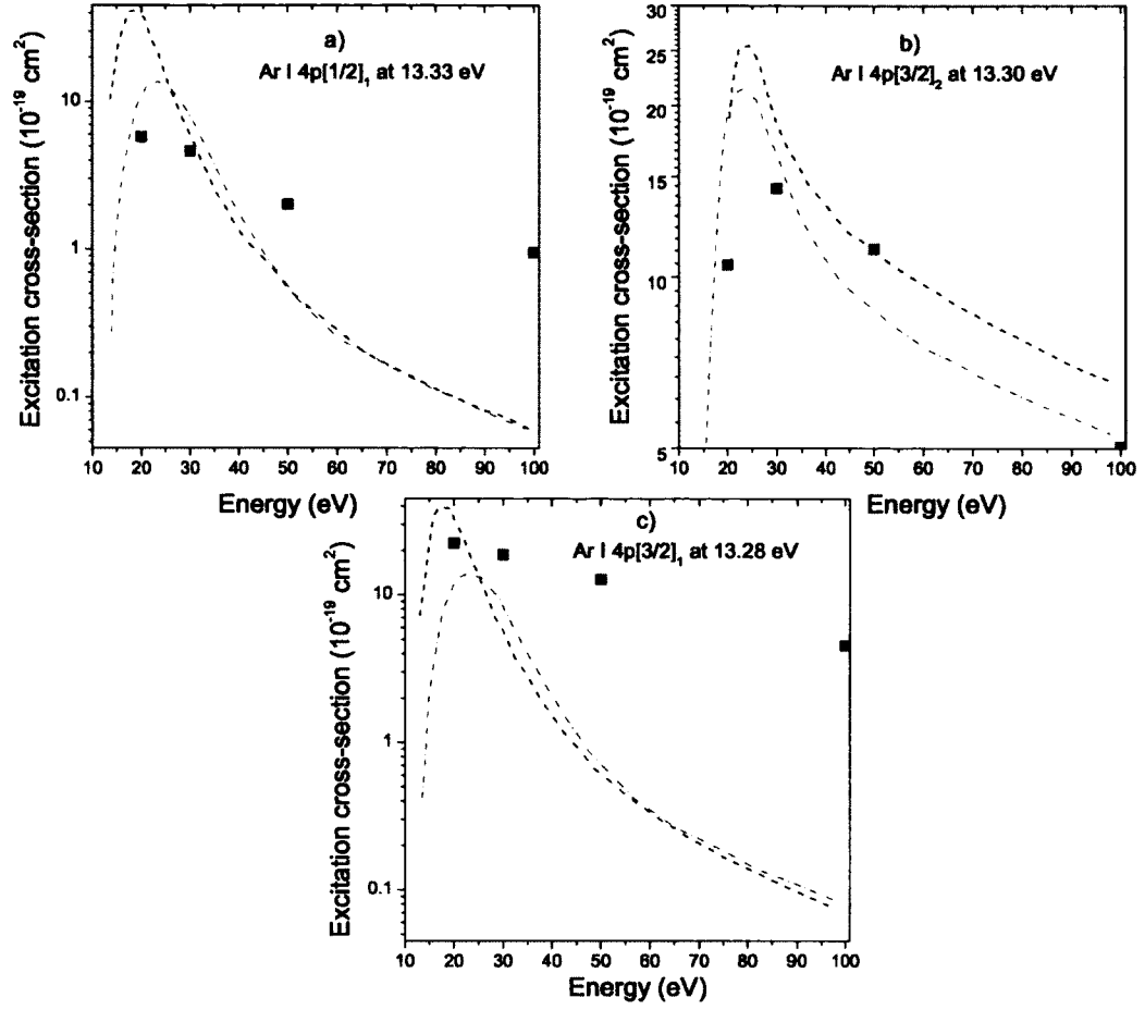
FIG. 2. Electron impact excitation cross-sections from Ar I ground state to Ar I a) 4p [1/2]_1 , b) 4p [3/2]_2 , and c) 4p [3/2]_1 states. Dashed lines present theoretical predictions from Ref. [24], and dots present theoretical predictions from Ref. [25]. Experimental results from Ref. [22,23] are connected with straight lines for better visualisation.
