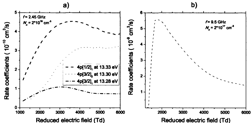
FIG. 15. Rate coefficient for electron impact excitation from ground state to excited a) 4p levels of Ar I and b) ( N_2(C^3\Pi_u) ) level dependence on reduced electric field using strong field approximation.
