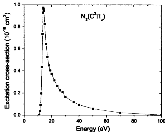
FIG. 4. Electron impact excitation cross-sections from N_2 ground state to N_2(C^3\Pi_u) state [20]. Experimental results are connected with straight lines for better visualization.
