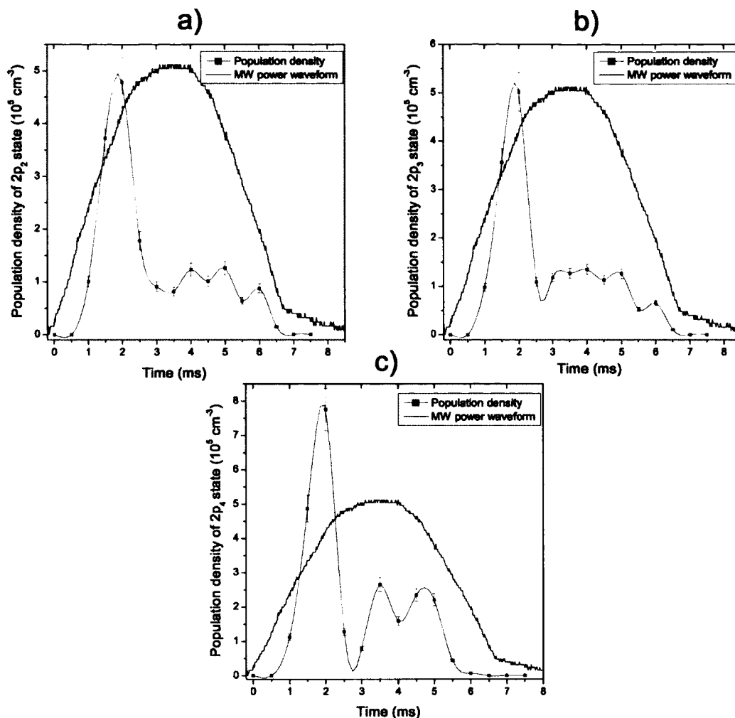
FIG. 61. Time dependence of the population densities inside the power sine signal at 2.3 Torr of the Ar I: a) 2p_2 state, b) 2p_3 state, and c) 2p_4 state. The experimental results are connected with the smoothed fitted line.
