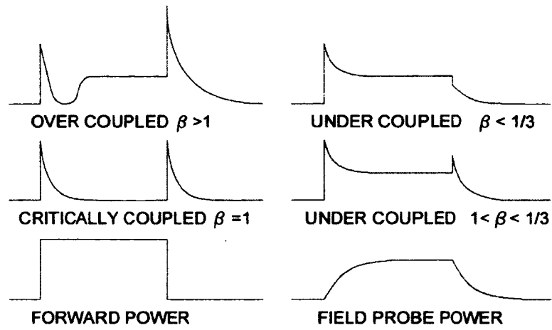
FIG. 144. Wave forms of incident and reflected power.
