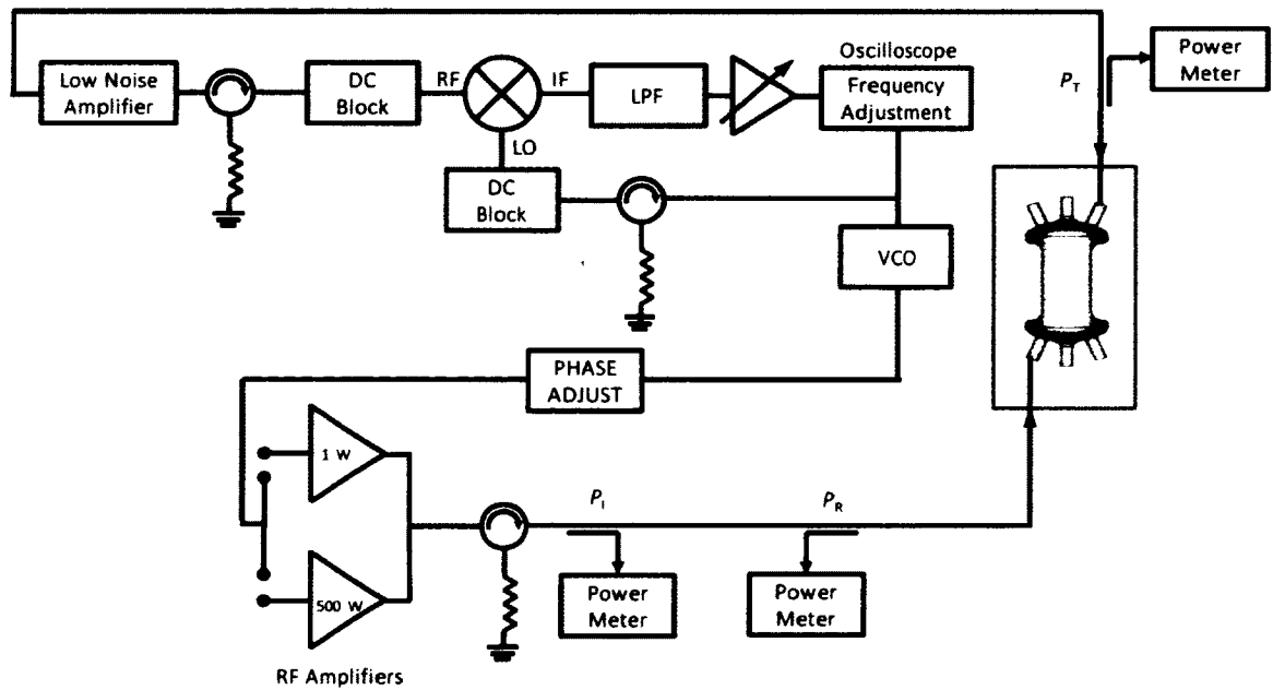
FIG. 145. Schematic of the rf system used for the Q_0 vs. field measurements.
