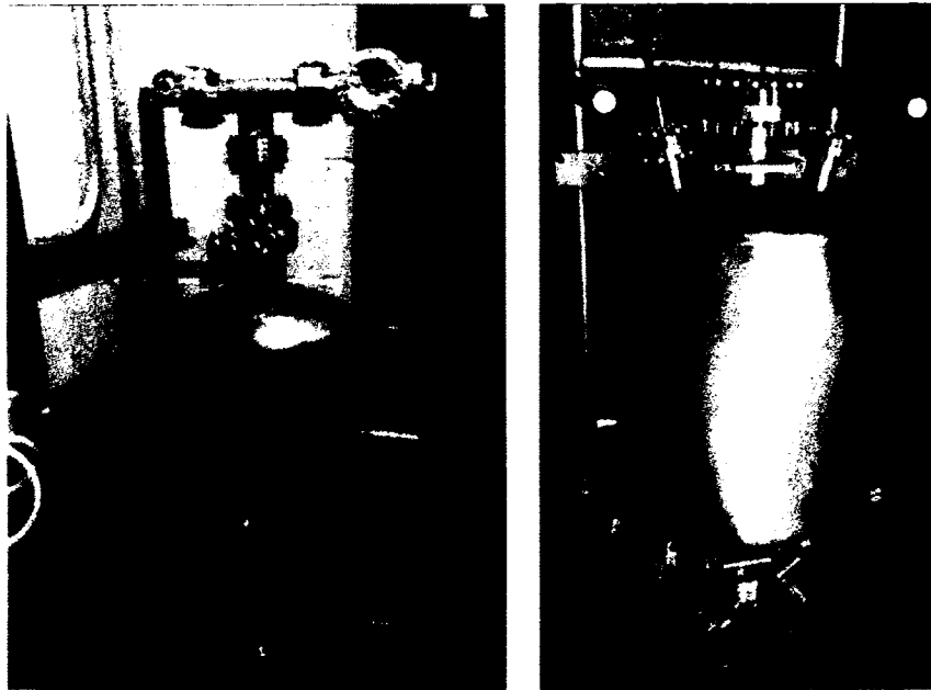
FIG. 140. 499 MHz (left) and 400 MHz (right) cavities assembled on the test stands.
