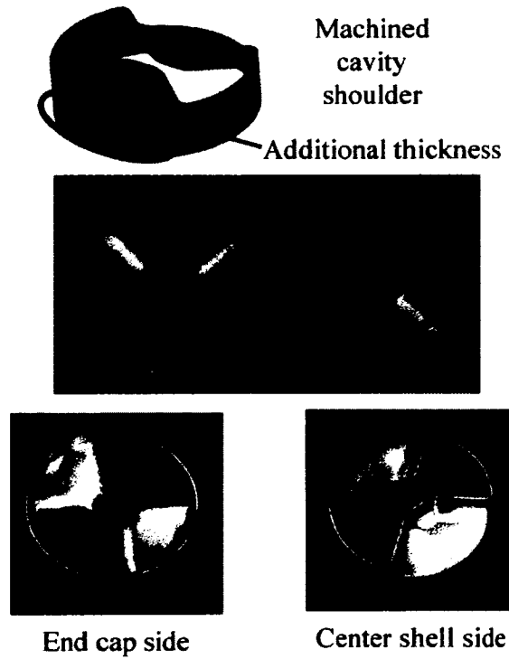
FIG. 122. Machined shoulder block of the 499 MHz cavity.
