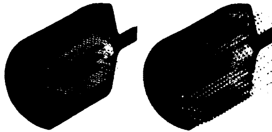
FIG. 64. Electric (left) and magnetic (right) field profile of the parallel-bar design with curved loading elements.
