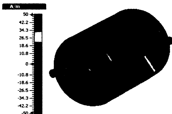
FIG. 156. Surface magnetic field on beam and coupler ports at a energy content of 1 J.
