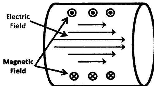
FIG. 1. Electric and magnetic fields of the TM_{010} mode in a cylindrical cavity.
