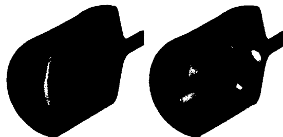
FIG. 65. Surface electric (left) and magnetic (right) field of the parallel-bar design with curved loading elements.
