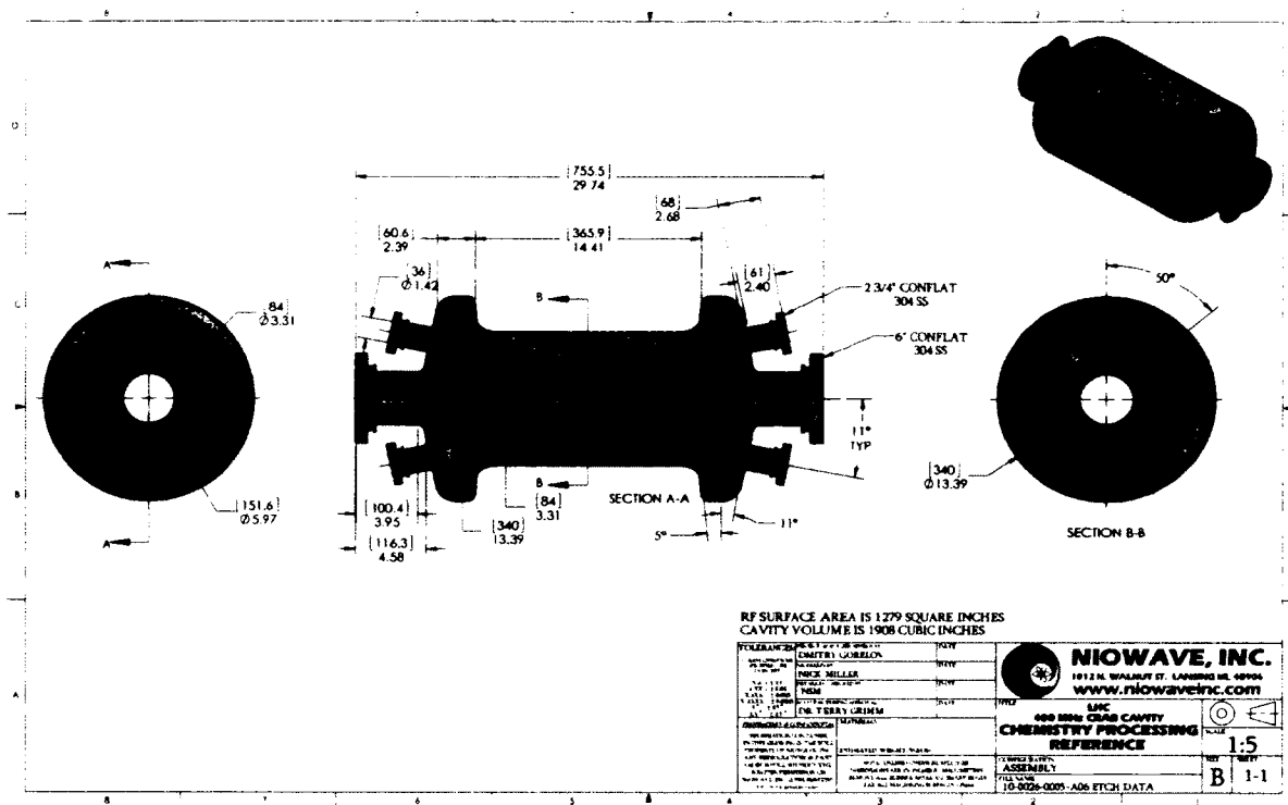
FIG. 126. Fabrication drawing of the 400 MHz rf-dipole cavity.
