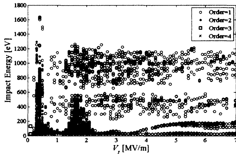
FIG. 114. Electron impact energy in the 400 MHz rf-dipole cavity with varying transverse voltage.
