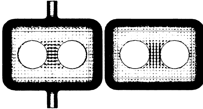
FIG. 31. Electric field (left) on the mid plane and magnetic field (right) on the top plane for the fundamental deflecting mode.
