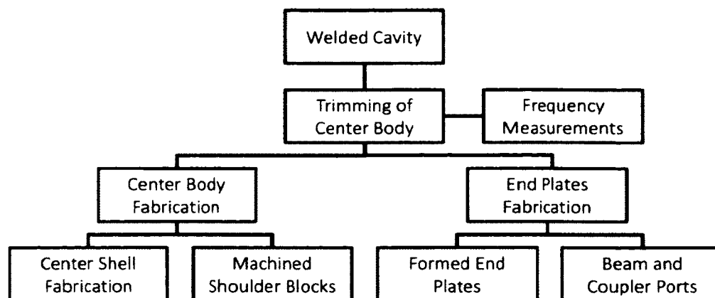
FIG. 118. Fabrication sequence of the 499 MHz rf-dipole cavity.
