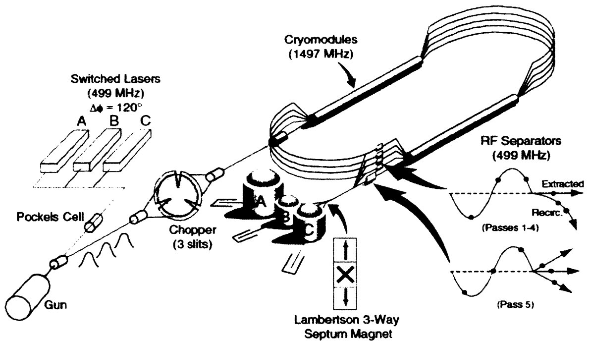
FIG. 20. Schematic of CEBAF accelerator.
