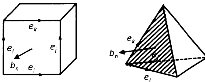
FIG. 29. A single meshing element in hexahedral (left) and tetrahedral (right) type mesh.
