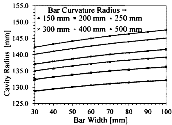
FIG. 61. Cavity radius with varying bar width and radius of bar curvature for race-track-shaped parallel bars.
