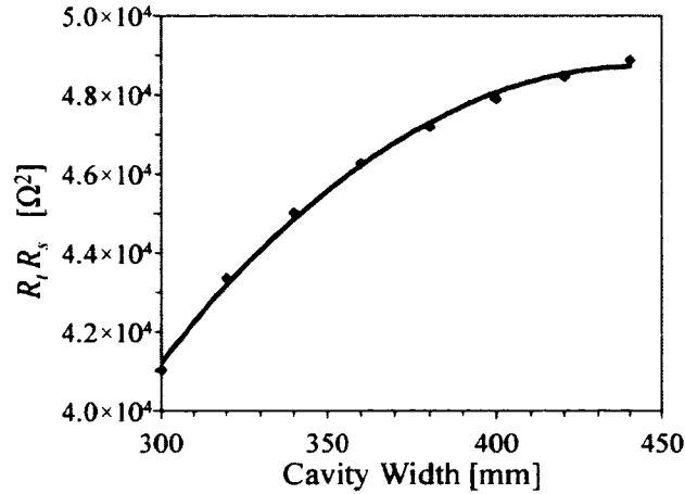
FIG. 43. Product of transverse shunt impedance ( R_t ) and surface resistance ( R_s ) with varying cavity width of parallel-bar design with rectangular-shaped outer conductor and cylindrical loading elements.
