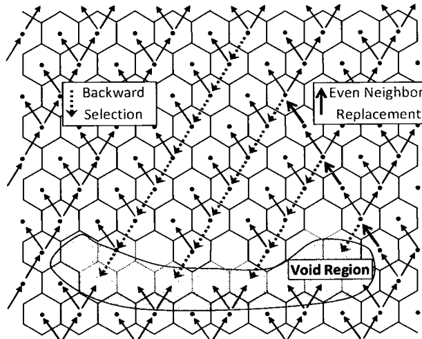
FIG. 13: Void recovery using even neighbor replacement/backward selection
