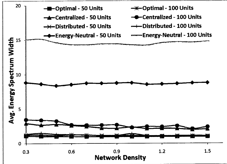
FIG. 31: Avg. width of energy spectrum for different initial energy levels
