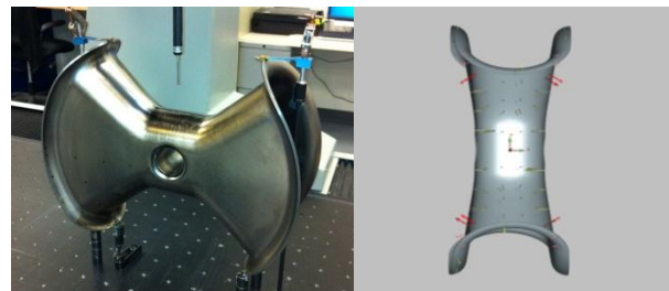
Figure 2: Welded spoke and CMM results showing deviations from the cavity model.
