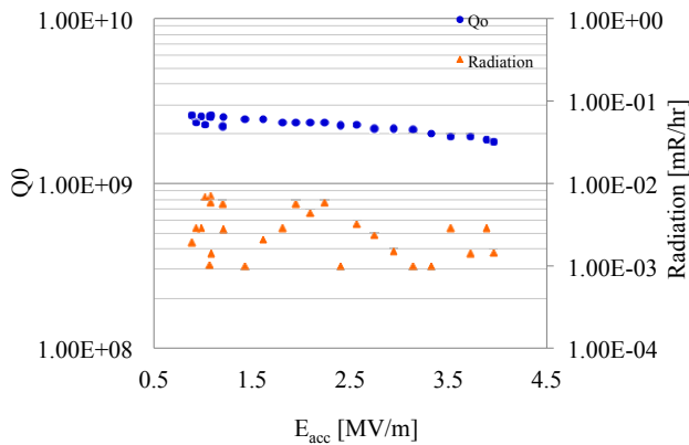
Figure 7: High power test results at 4.3K.
