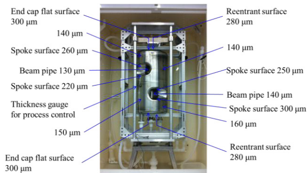
Figure 6: BCP set-up and thickness measurement results.
