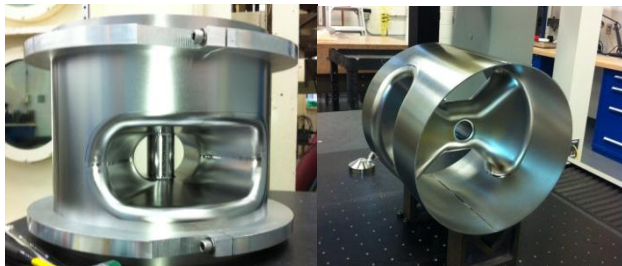
Figure 3: Weld fit-up and completed spoke-outer conductor subassembly
