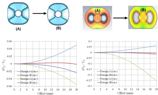
Figure 18: Field non uniformity of rf-dipole cavity (left) and 4-rod cavity (right).
