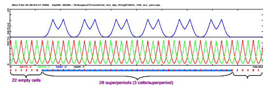
Figure 2. ELIC electron collider ring Lattice.
