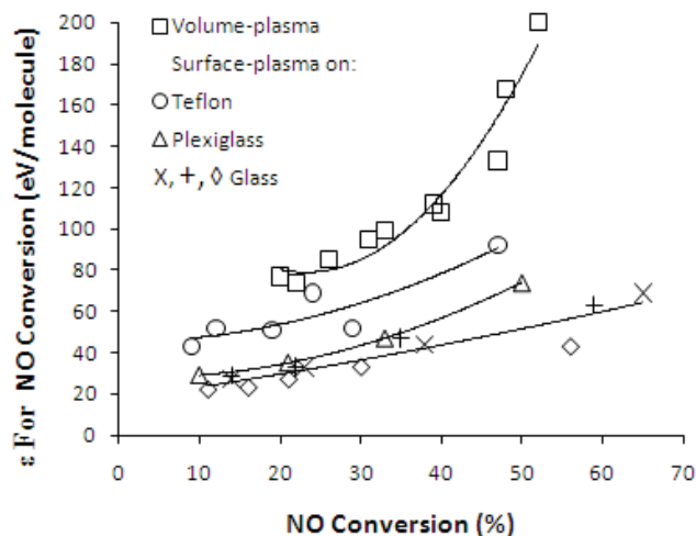
Fig. 9. Energy cost ( \epsilon ) versus NO conversion (NO balance N_2 ). The points ( \square , \circ , \Delta , x , + , & \diamond ) represent experimental values and curves serve as a visual guide of the trends. The electrode lengths were 16.5 cm, the gaps between anode and cathode were 3.8 cm, and thickness of the spacer was 0.2 cm in the surface plasma reactors).
