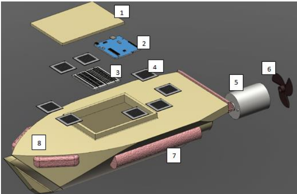
Figure 2: Explode state and basic parts of a solar boat concept 28
