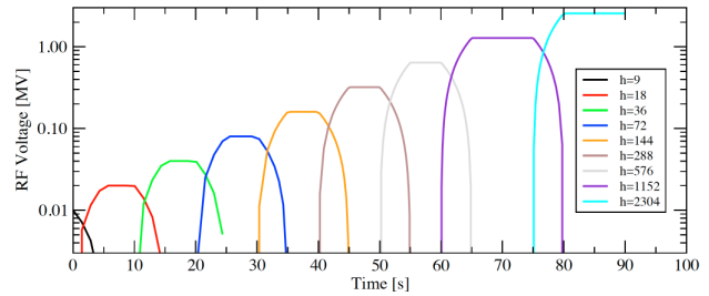
Figure 3: RF voltages used for initial JLEIC multiple 1:2 splitting simulations, showing voltage doubling with each successive harmonic.
