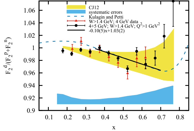
FIG. 2. (Color online) The deuteron EMC ratio R_{\text{EMC}}^d = F_2^d / (F_2^n + F_2^p) as extracted from the BONuS data. Total systematic uncertainties are shown as a band arbitrarily positioned at 0.91 (blue). The yellow band shows the CJ12 [49] limits expected from their nuclear models. The black points are the combined 4- and 5-GeV data, whereas the red points are the 4-GeV data alone. The dashed blue line shows the calculations of Ref. [36]. The solid line (black) is the fit to the black points for 0.35 < x < 0.7 .
