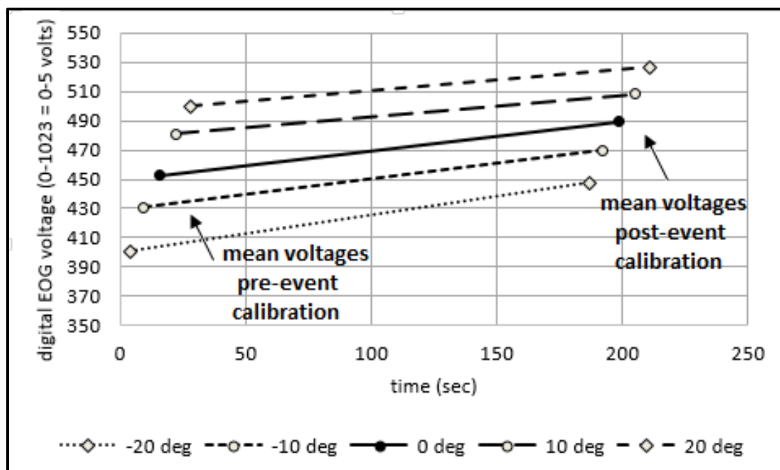
Fig. 32. Sample Mean Voltages of Pre- and Post-Event Calibration Baseline Drift.
