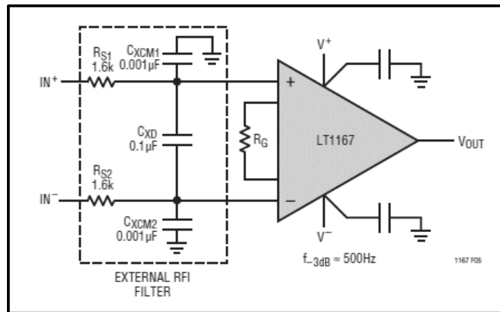
Fig. 22. EOG Amplifier Circuit Configuration [171].
