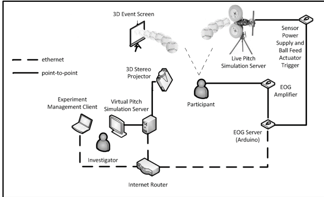
Fig. 14. Simulation Environment and EOG System Client-Server Architecture.
