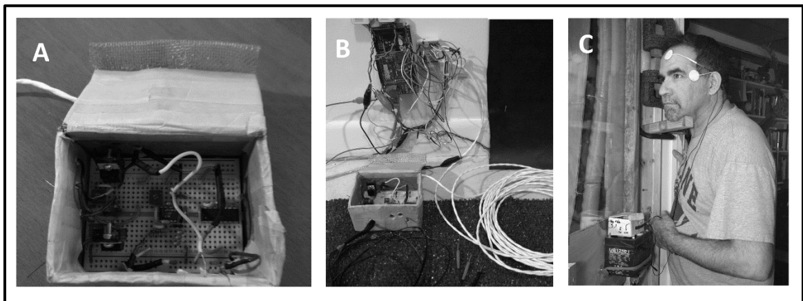
Fig. 23. EOG Server: A – Amplifier, B – Amplifier Interfaced to Microcontroller, and C – Interfaced to Microcontroller and Participant.
