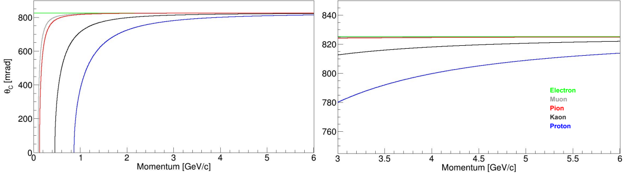
FIG. 8: Particle momentum (in GeV/c) versus Cherenkov angle (in mrad) for different particle species in fused silica ( n \approx 1.473 ). While the full range (left) makes it seem as if separation between heavier species becomes more and more challenging, zooming in (right) shows that it is indeed possible to separate protons, kaons, and pions even at higher particle momentum.
