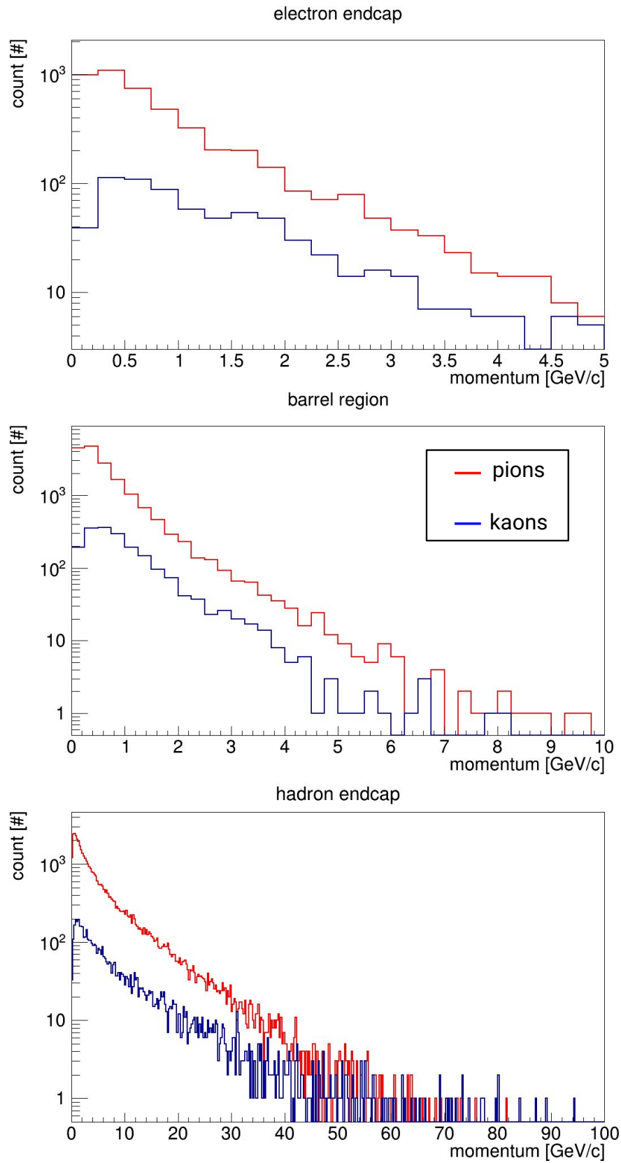
FIG. 6: Momentum distributions for pions (red) and kaons (blue) in the electron endcap (top), barrel region (middle), and hadron endcap (bottom). Plots were produced using the pythia simulation package for DIS events corresponding to collisions between 10 GeV electrons and 100 GeV protons, a common BNL/JLab kinematic, shown for a bin of 10 < Q^2 < 100 \text{ GeV}^2 [14].
