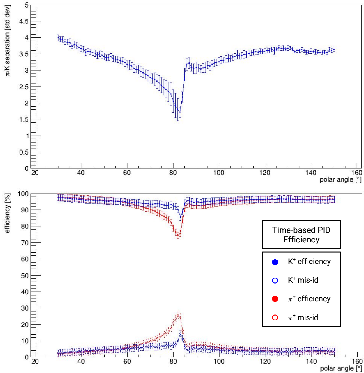
FIG. 33: Simulated performance of the DIRC at EIC baseline design. Top: Separation power as a function of polar angle for 6 GeV/c pions and kaons using time-based reconstruction. Bottom: Efficiency (solid circles) of PID as a function of polar angle for pions (red) and kaons (blue) along with the mis-identification rate (open circles).
