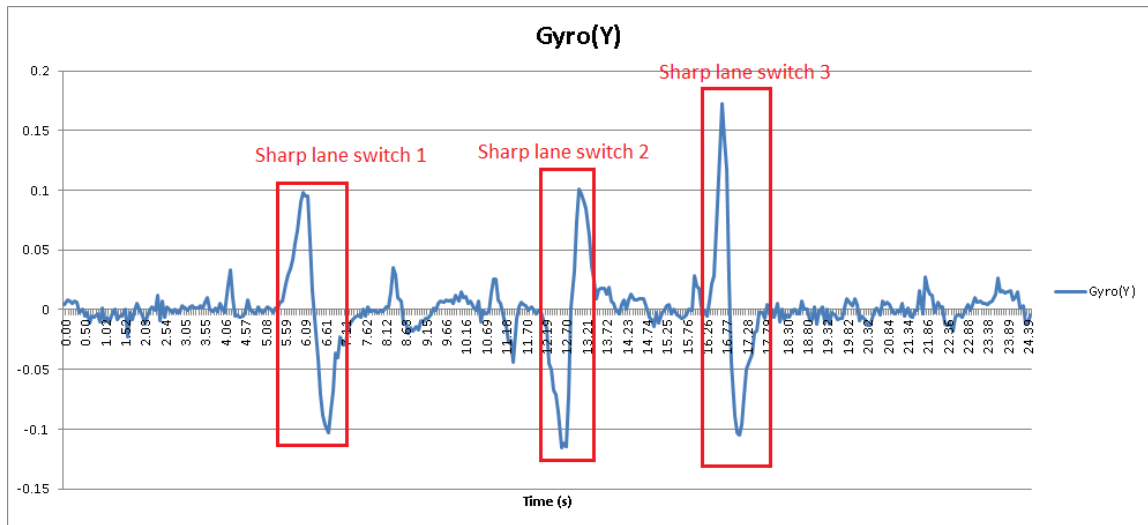
FIG. 34: Lane switches using gyroscope
