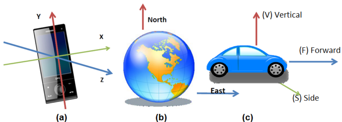
FIG. 17: Coordinate systems. (a) Device Coordinate System, (b) Earth Coordinate System, (c) Vehicle Coordinate System.
