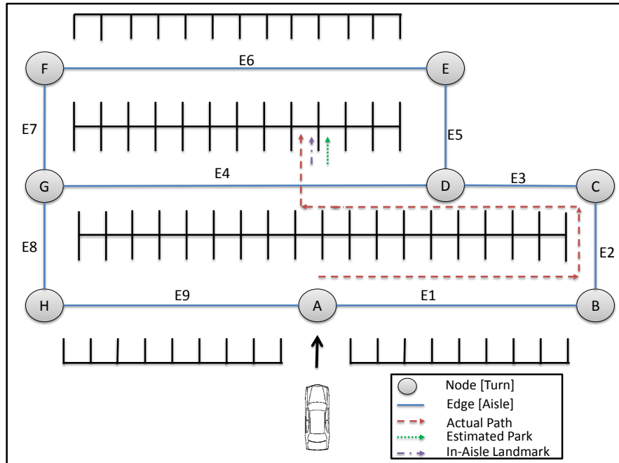
FIG. 43: Parking-lot diagram
