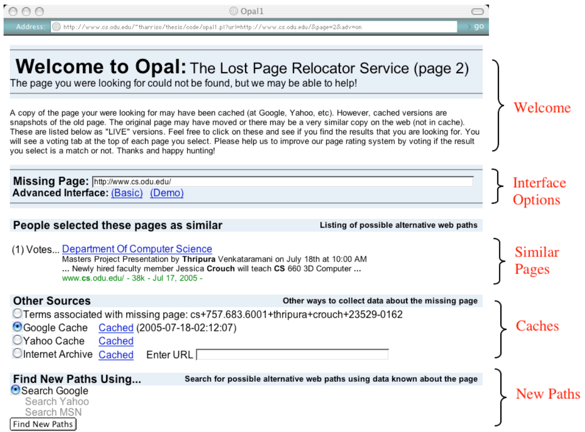
Fig. 10. GUI components.
