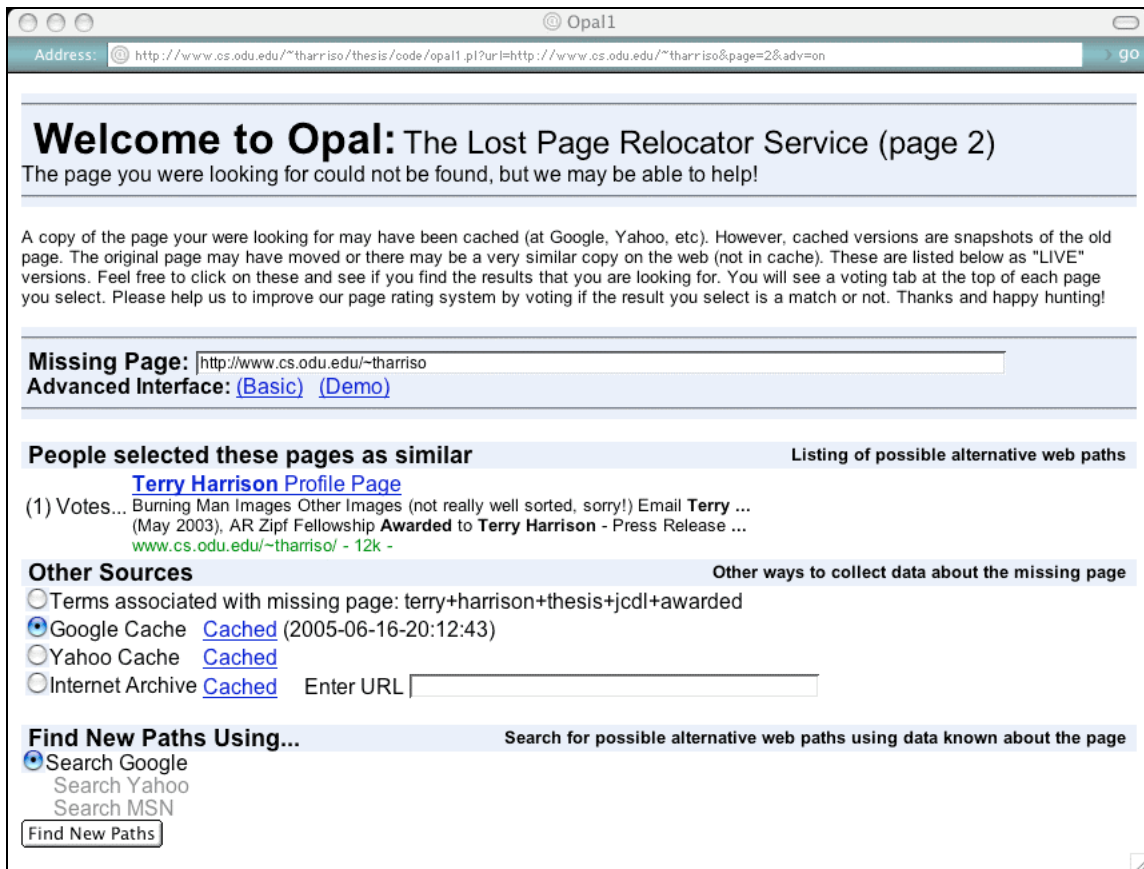
Fig. 14. Advanced interface.
