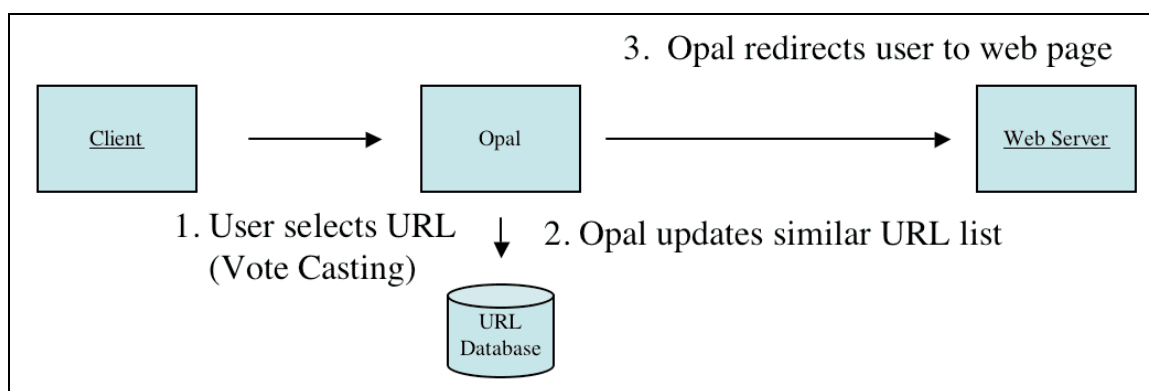
Fig. 34. Voting mechanism.
