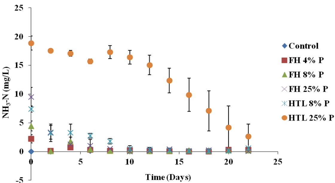
Figure 8. NH 3 -N values (average for each treatment) for the Scenedesmus cultivation using FH Hydrolysate and HTL AP study.
